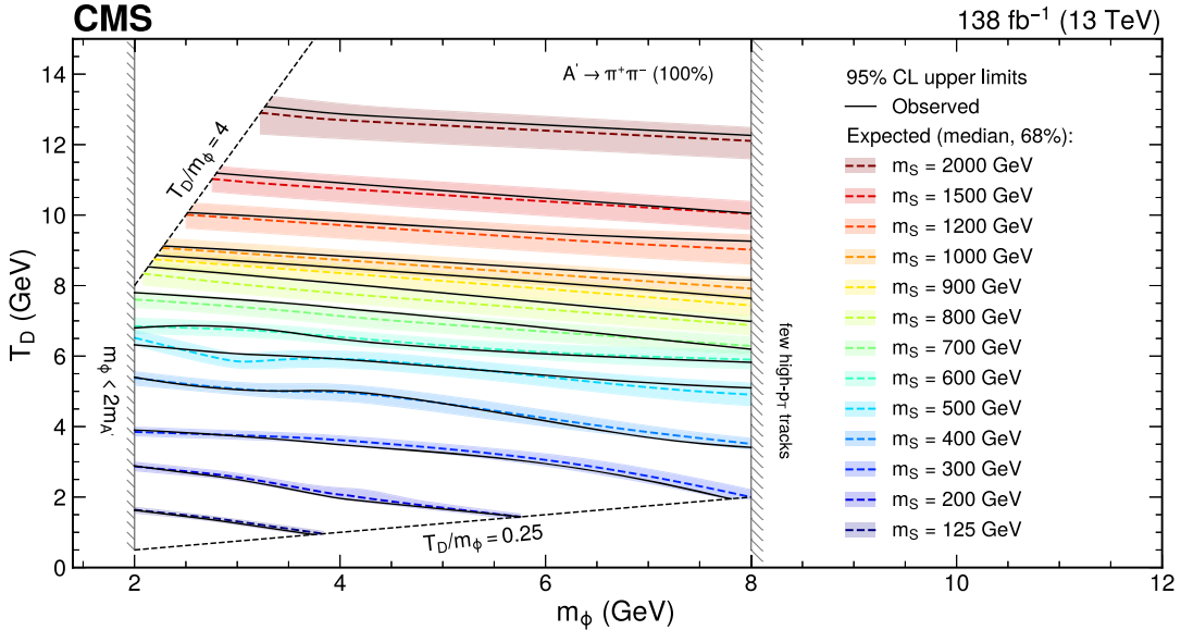
FIG. 4. The observed and expected exclusions for the nominal S cross section in the plane of m_\phi and T_D , for various m_S values, for the case m_{A'} = 1.0 GeV ( A' \rightarrow \pi^+\pi^- with B = 100\% ). The regions below the observed limits are excluded.
