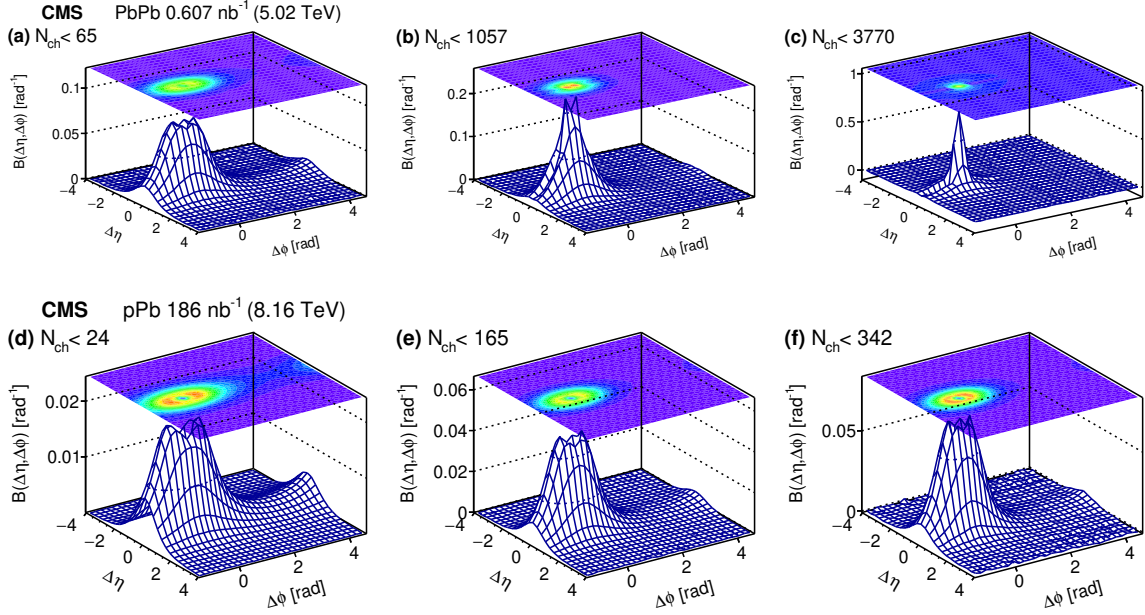
Figure 1. The balance function is shown in terms of \Delta\eta and \Delta\phi in PbPb collisions at \sqrt{s_{\text{NN}}} = 5.02 TeV (upper panels) and for p\text{Pb} collisions at 8.16 TeV (lower panels). From left to right, the results are shown for the lowest to highest multiplicity classes in PbPb and p\text{Pb} collisions. The trigger and associated particles in PbPb ( p\text{Pb} ) collisions satisfy the condition 0.5(0.4) < p_{\text{T,asso}} < p_{\text{T,trig}} < 2.0 GeV.
