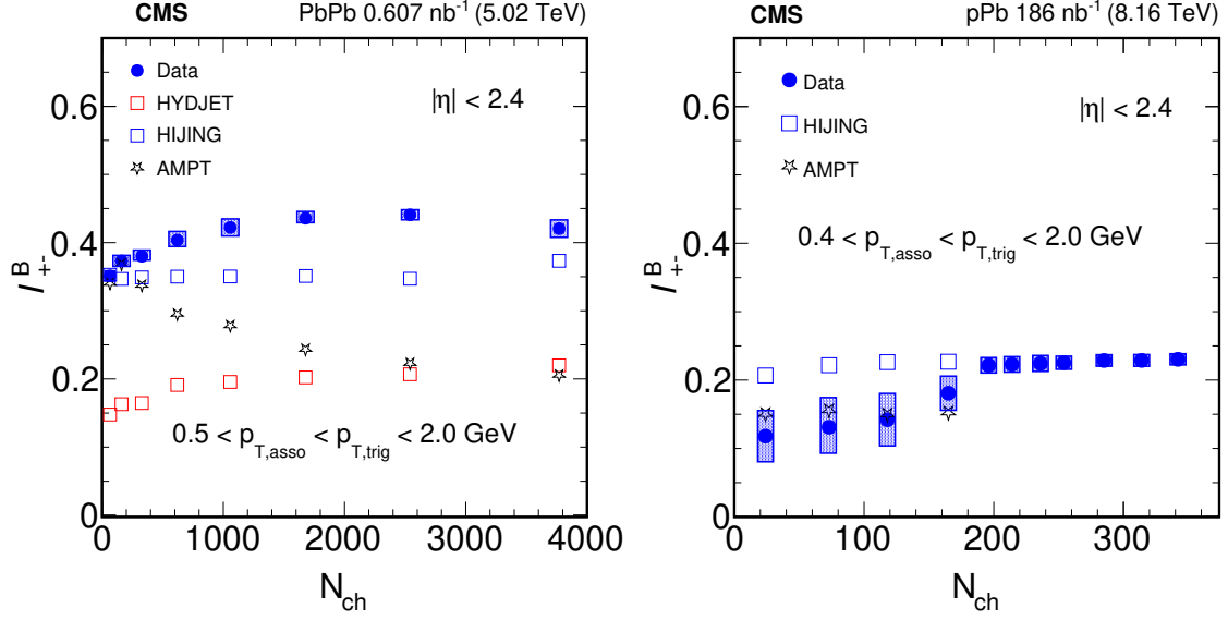
Figure 5. The integral of the balance functions ( I_{+-}^B ) in PbPb collisions at \sqrt{s_{\text{NN}}} = 5.02 TeV (left) and in p\text{Pb} collisions at \sqrt{s_{\text{NN}}} = 8.16 TeV (right). The balancing partners fall within the specified pseudorapidity range ( |\eta| < 2.4 ) and have transverse momenta within the range of 0.5 < p_T < 2.0 GeV (for PbPb) and 0.4 < p_T < 2.0 GeV (for p\text{Pb} ). The statistical uncertainties in the data points are smaller than the marker size and rectangular boxes indicate the systematic uncertainties.
