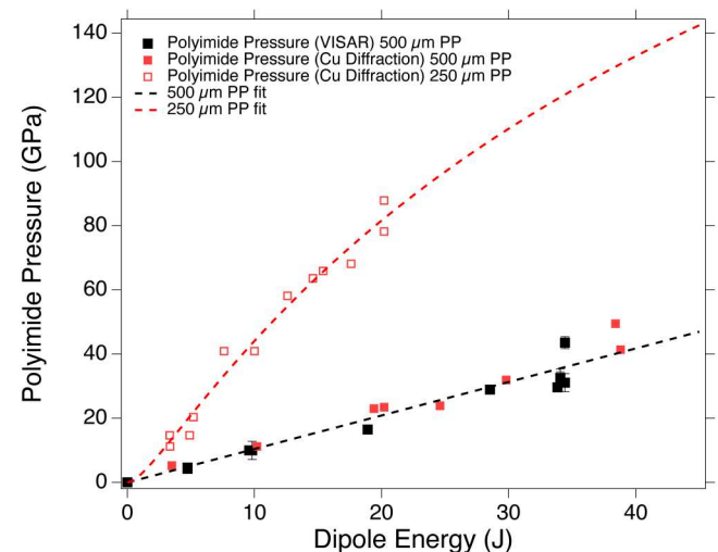
FIG. 3. Polyimide pressure as a function of laser energy for 500 and 250\text{ }\mu\text{m} phase plates (PPs). This relation was determined by two independent methods: using impedance matching from VISAR traces from polyimide-LiF targets (black); using impedance matching from Cu diffraction data from polyimide-Cu targets (red).
