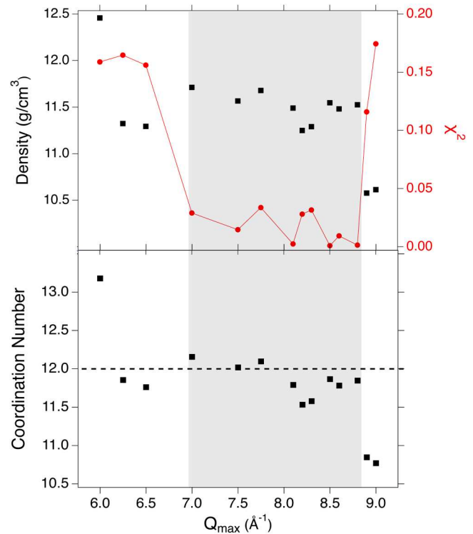
FIG. 8. Effect of Q_{\max} on optimization—shot 831. Density and \chi^2 (top) and coordination number (bottom) was determined as a function of Q_{\max} . The figure of merit \chi^2 (red) is minimized between 7.0 and 8.8 \text{\AA}^{-1} .
