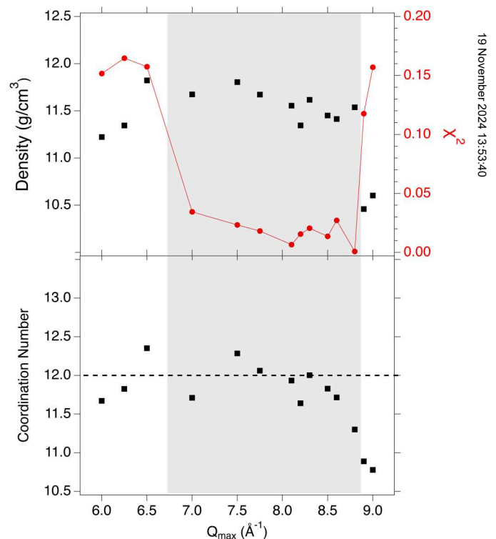
FIG. 6. Effect of Q_{\text{max}} on optimization—shot 826. Density and \chi^2 (top) and coordination number (bottom) as determined as a function of Q_{\text{max}} . The figure of merit \chi^2 (red) is minimized between 7.0 and 8.8 \text{ \AA}^{-1} .
