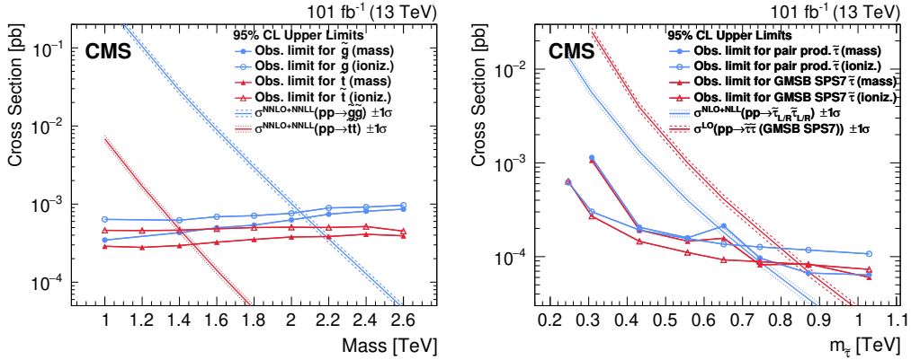
Figure 6: Cross section limits for \tilde{g} (blue circles) and \tilde{t} R-hadrons (red triangles) on the left and for the direct pair production of \tilde{\tau} (blue circles) and within the GMSB SPS7 model (red triangles) on the right. The results obtained with the ionization method are displayed with open symbols, while the symbols for the mass method are filled. Corresponding theoretical predictions are shown using the same color code.
