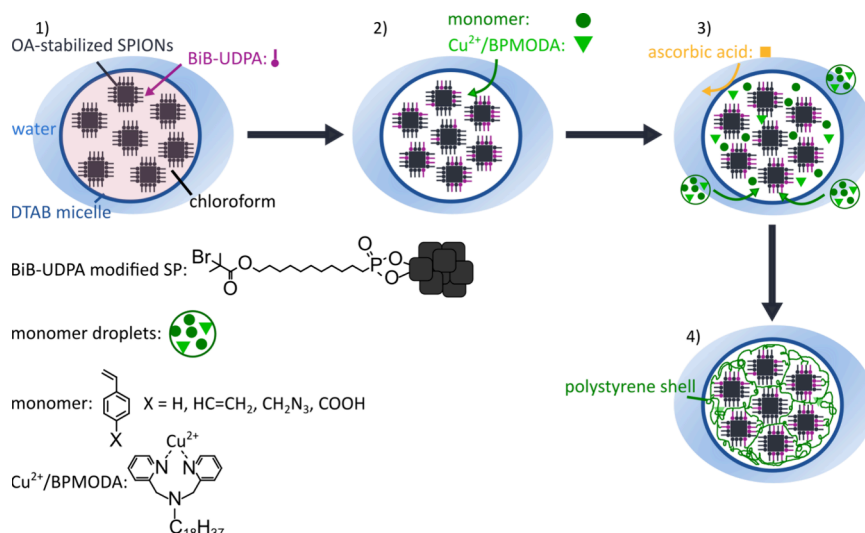
Figure 1. Strategy for the surface-grafted polymer encapsulation of SPs from SPIONs: (1) Ligand exchange of oleic acid (OA) for BiB-UDPA. (2) Addition of the catalyst \text{Cu}^{2+}/\text{BPMODA} and the monomer [e.g., styrene and divinylbenzene (DVB)]. (3) Reduction of the catalyst and initiation of the ATRP using ascorbic acid. (4) Controlled ATRP growth of the polymer shell.
