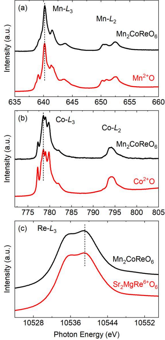
Figure 2. XAS at the (a) Mn- L_{2,3} , (b) Co- L_{2,3} , and (c) Re- L_3 edges of MCRO. The XAS of MnO, CoO and Sr 2 MgReO 6 are displayed as Mn 2+ , Co 2+ and Re 6+ references, respectively.
