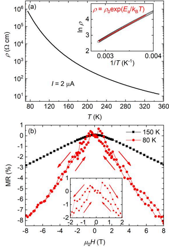
Figure 8. (a) Temperature dependent resistivity of MCRO. The inset displays the experimental data (black circles) and the thermal activation model fitting with formula \rho = \rho_0 \times \exp(E_a/k_B T) in the temperature range 260–350 K. (b) Field dependent magnetoresistance of MCRO at 150 K and 80 K. The inset depicts the region of \pm 2 T.
