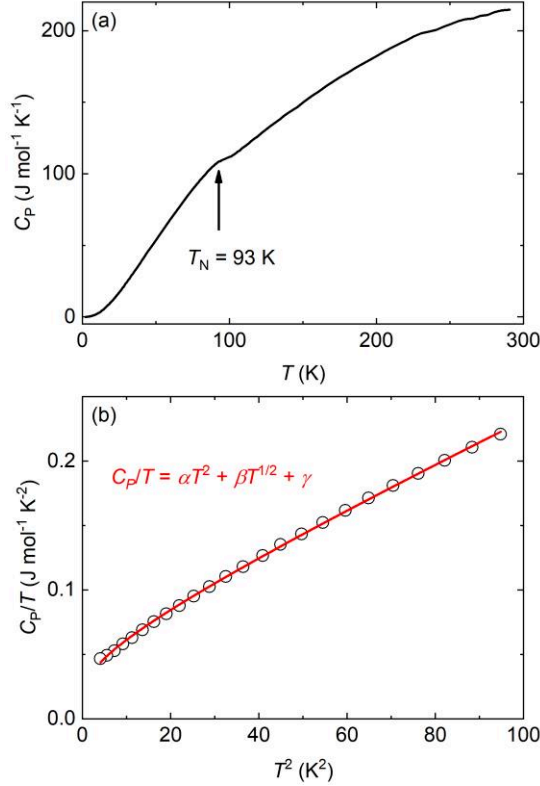
Figure 4. (a) Temperature dependent heat capacity of MCRO. (b) Experimental heat capacity below 10 K (black circles) and the fitting with formula C_P/T = \alpha T^2 + \beta T^{1/2} + \gamma (red line).
