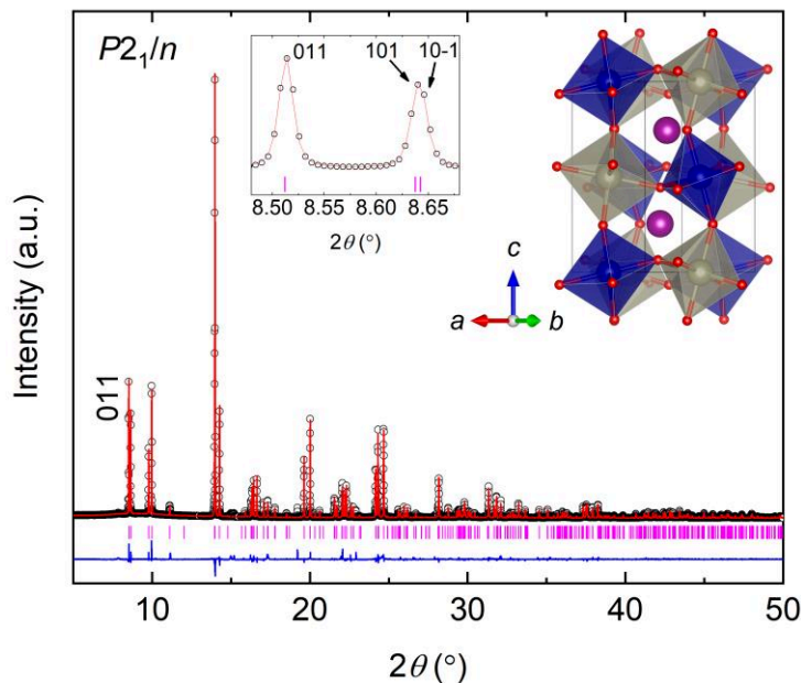
Figure 1. SXRD pattern and Rietveld refinement of MCRO. The black circles, red lines and blue lines indicate the observed, calculated and difference, respectively. The magenta ticks indicate the allowed Bragg reflections for space group P2_1/n . The inset in the middle displays the SXRD pattern near the (011) diffraction peaks. The inset at the right side displays the crystal structure of MCRO. Mn, Co, Re and O are shown in purple, blue, grey and red, respectively.
