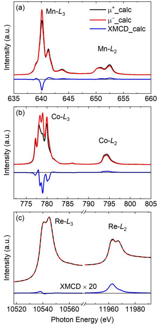
Figure 6. Calculated XMCD spectra at the (a) \text{Mn-}L_{2,3} , (b) \text{Co-}L_{2,3} , and (c) \text{Re-}L_{2,3} edges of MCRO. The XAS with light polarization parallel ( \mu^+ , black lines) and antiparallel ( \mu^- , red lines) to the magnetic field are shown. The blue lines are the XMCD ( \mu^+ - \mu^- ) spectra.
