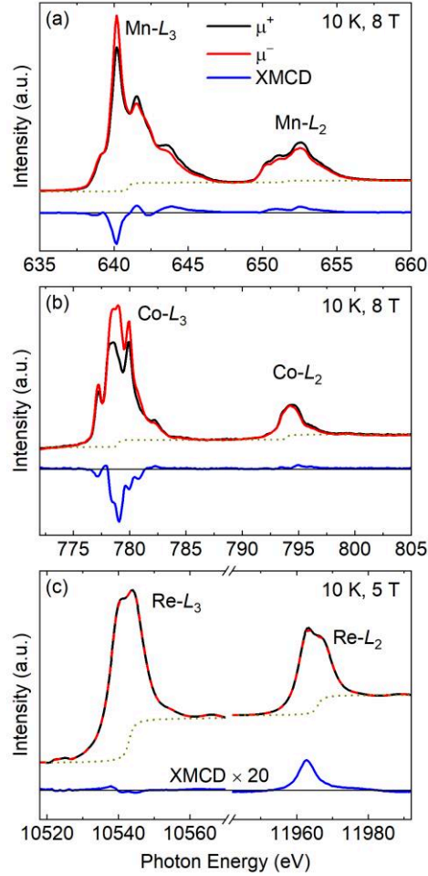
Figure 5. XMCD spectra at the (a) Mn- L_{2,3} , (b) Co- L_{2,3} , and (c) Re- L_{2,3} edges of MCRO. The XAS with light polarization parallel ( \mu^+ , black lines) and antiparallel ( \mu^- , red lines) to the magnetic field are shown. The blue lines are the XMCD ( \mu^+ - \mu^- ) spectra. The dashed lines indicate the edge jump.
