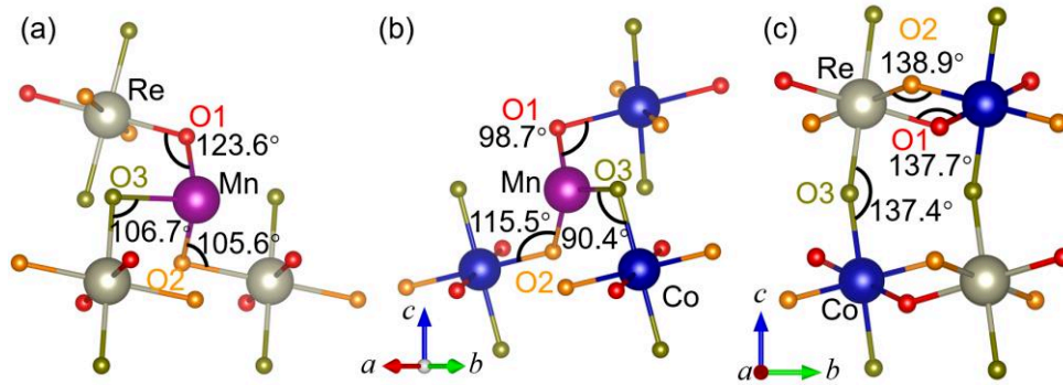
Figure 7. The bond angles of (a) Mn-O-Re, (b) Mn-O-Co and (c) Co-O-Re. The Mn, Co and Re ions are shown in purple, blue and grey, respectively. The different O sites are shown in red, orange and brown, respectively.
