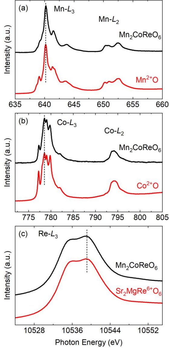
Figure 2. XAS at the (a) Mn- L_{2,3} , (b) Co- L_{2,3} , and (c) Re- L_3 edges of MCRO. The XAS of MnO, CoO and \text{Sr}_2\text{MgReO}_6 are displayed as \text{Mn}^{2+} , \text{Co}^{2+} and \text{Re}^{6+} references, respectively.
