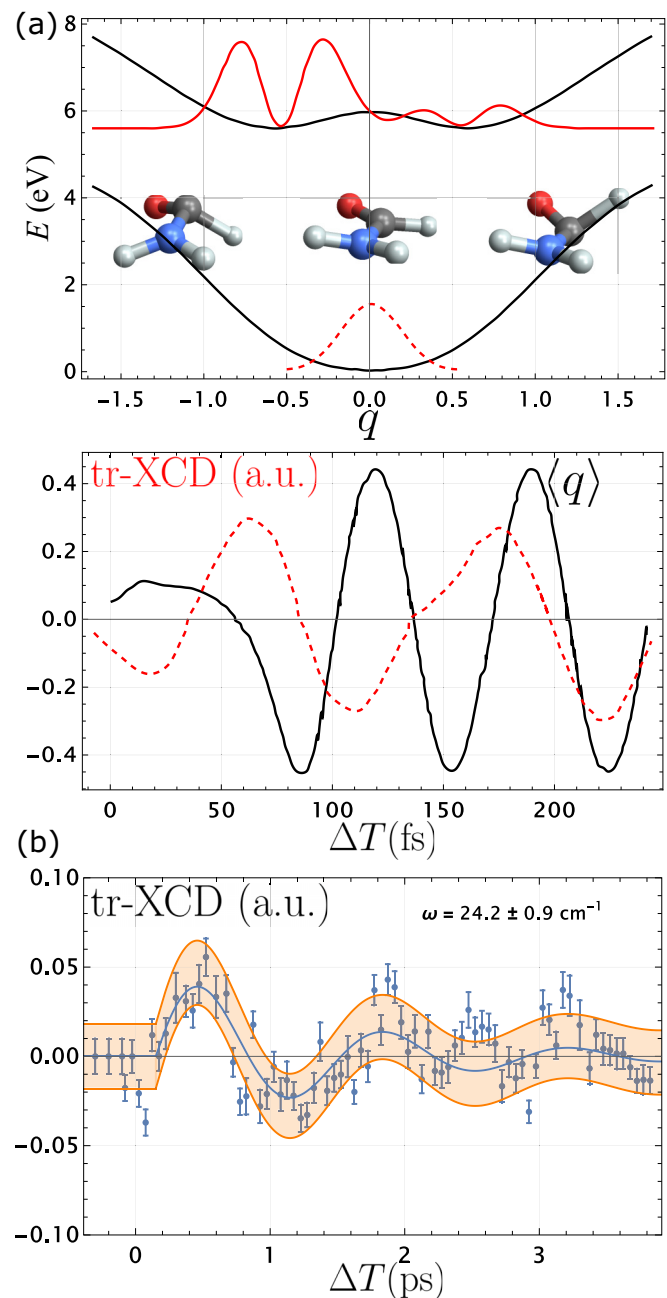
FIG. 32. (a) The formamide molecule is achiral in its ground state and becomes chiral in its first excited state through pyramidalization. When pumped by circularly polarized UV light, the nuclear wave packet oscillates between the two enantiomers (top panel). The tr-XCD signal (middle panel, dashed, red) follows closely the nuclear wave-packet center of mass dynamics (solid, black) [175] and is a sensitive probe of the local chiral nuclear dynamics. (b) tr-XCD can also be used as a local windows into chiral vibrational dynamics. In the lower panel, low-lying vibrational excitations are pumped by a UV Raman process [434] and tr-XCD is used as a local probe of chiral nuclear dynamics.
