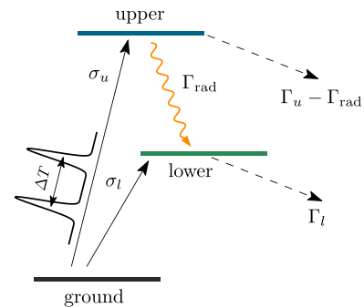
FIG. 2. Level scheme used in the numerical simulations with the following parameters, adapted to the case of the Cu-like K\alpha transition of \omega_0 = 8.048 keV: decay rates \Gamma_u = 2.1 \text{ fs}^{-1} and \Gamma_l = 0.9 \text{ fs}^{-1} , the rate of spontaneous emission \Gamma_{\text{rad}} = 0.6 \text{ fs}^{-1} , and photoionization cross-sections \sigma_u = 25.3 \text{ Kb} and \sigma_l = 9.5 \text{ Kb} . A fraction of this fluorescence (this fraction is defined in Sec. VB) travels through the sample, inducing superfluorescence. In reality, \sigma_l is considerably lower for Cu. We have increased this parameter to induce more dynamics to the lower state. The atomic concentration is assumed as n = 85.0 \text{ nm}^{-3} .
