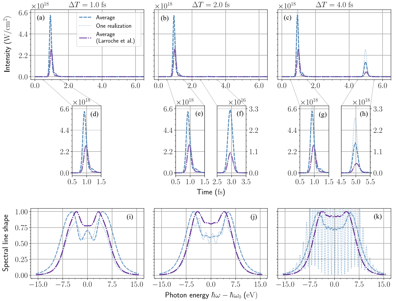
FIG. 6. Temporal (a)–(c) and normalized spectral (i)–(k) intensities in the saturation regime at a length of z = 14.3L_g ( 16.6 \mu\text{m} ) for separations of \Delta T = 1.0, 2.0 , and 4.0 fs between the two pump pulses. The resulting two emission bursts differ drastically in their intensities; we show each burst in separate panels (d)–(h). The emission spectra feature the Autler-Townes splittings due to Rabi oscillations, and in the single-shot spectra, spectral fringes become apparent.
