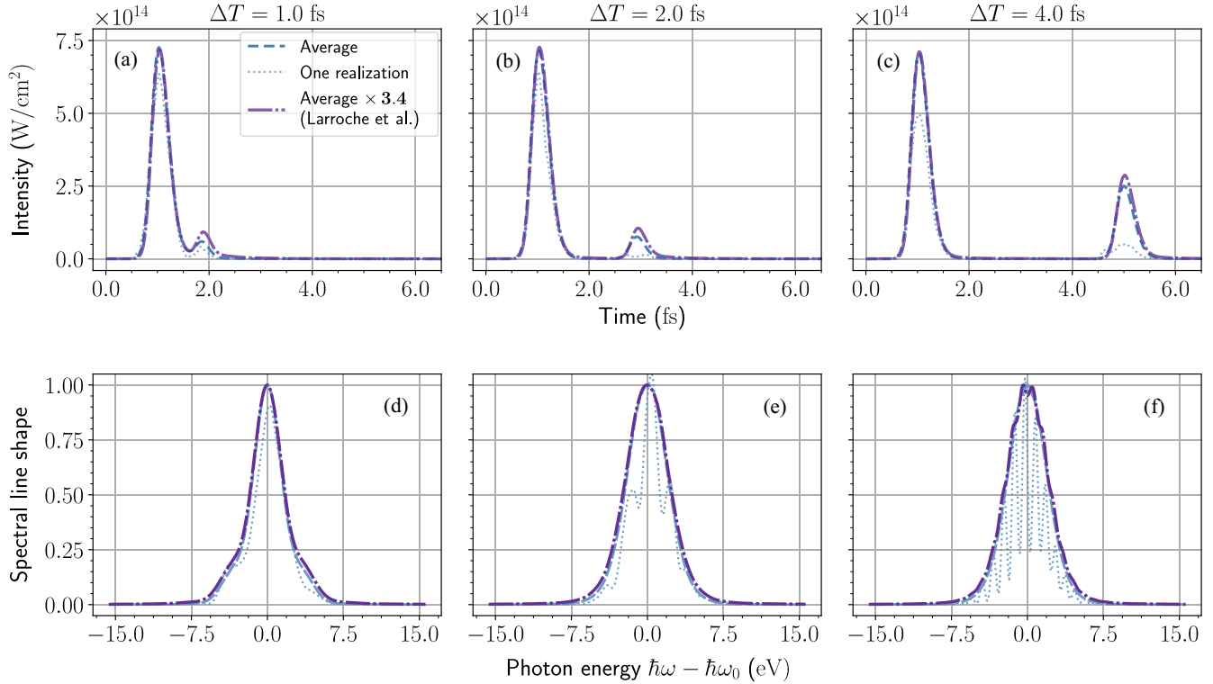
FIG. 5. Temporal (a)–(c) and normalized spectral (d)–(f) intensities of amplified spontaneous emission at a length of z = 3.0L_g ( 3.5 \mu\text{m} ) for separations of \Delta T = 1.0, 2.0 , and 4.0 fs between the two pump pulses. The average temporal intensities based on our (dashed blue line) and phenomenological (dash-dotted purple line) methodologies almost coincide when scaled to the same peak intensity (the purple curves have been scaled by a factor of 3.4). Similarly, the normalized average spectral intensities based on our estimation (dashed blue line), and on the phenomenological methodology (dash-dotted purple line), are almost identical. The dotted blue lines show single realizations, which exhibit a fringe pattern in the emitted spectrum due to the temporally separated two emission bursts.
