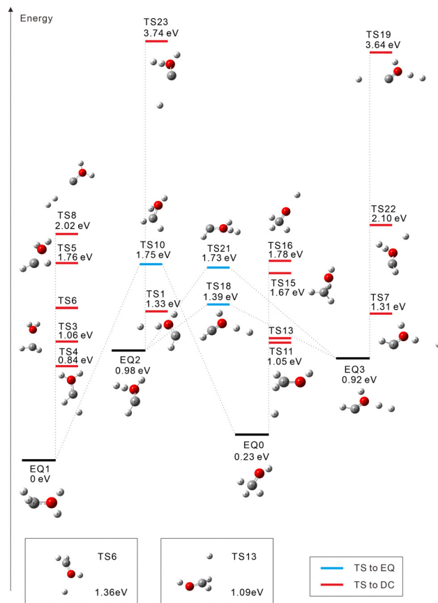
Fig. 2 Calculated isomerization and dissociation pathways for the triplet dication \text{CH}_3\text{OH}^{2+} (red: O, gray: C, and white: H). EQ/ i , TS/ i : equilibrium geometry and transition state, respectively. The energy difference from the neutral ground state to the dication EQ0 is calculated to be +30.34 eV for the triplet state (including the ZPVE correction). Due to space limitations, two TSs are shown in boxes.
