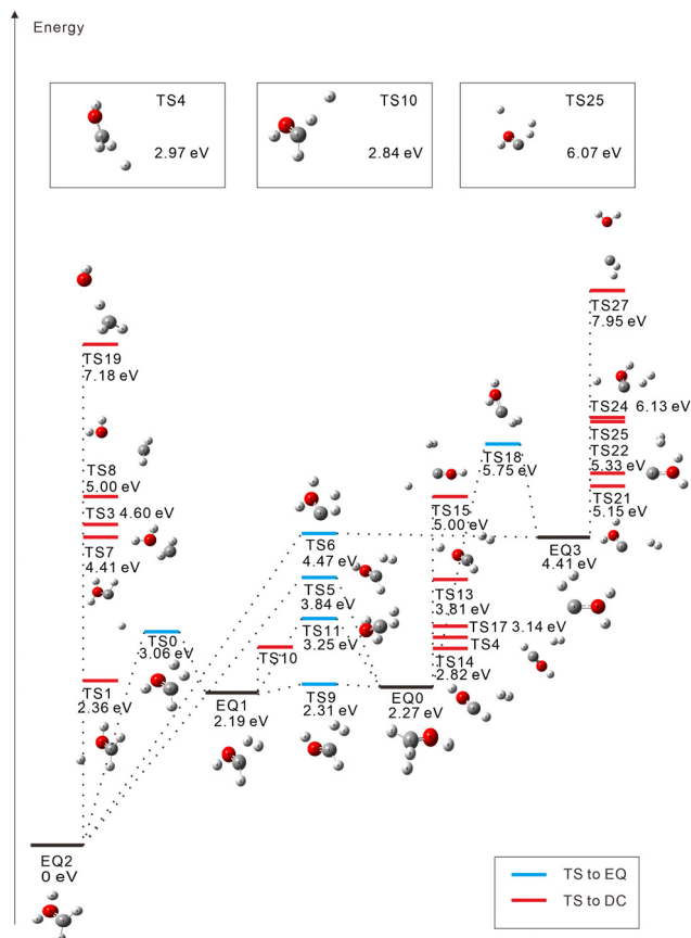
Fig. 1 Calculated isomerization and dissociation pathways for the singlet dication \text{CH}_3\text{OH}^{2+} (red: O, gray: C, and white: H). EQ/ i , TS/ i : equilibrium geometry and transition state, respectively. The energy difference from the neutral ground state to the dication EQ0 is calculated to be +28.59 eV for the singlet state (including the ZPVE correction). Due to space limitations, three TSs are shown in boxes.
