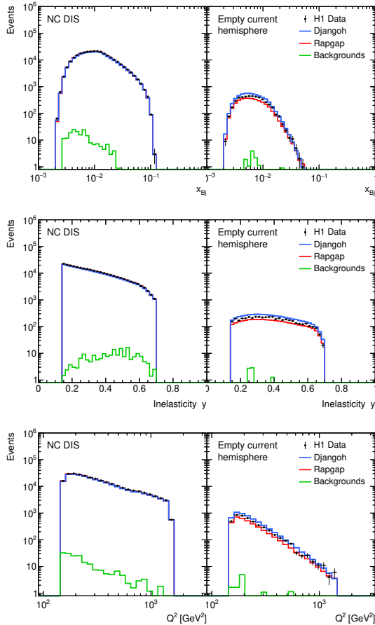
Fig. 3 Event distributions as functions of x_{\text{Bj}} (top), y (middle), and Q^2 (bottom) at the detector level in comparison with the simulated MC event samples from Djangoh and Rapgap that further include background events from photoproduction and lower Q^2 . The left panels display events after selection of all NC DIS events, and the right panels display events with an empty current hemisphere in the Breit frame.
