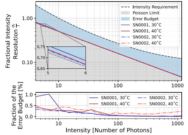
Fig. 26. Intensity resolution of fully calibrated modules with the SST requirement in black. The Poisson Limit is marked by the gray area. The performance of the whole SST camera must be in the blue area, defined as error budget as multiple components contribute to it. A quantum efficiency of 40% for the photomultipliers is assumed with a 3.37 mV pulse per photo electron conversion.
