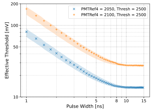
Fig. 11. The effective threshold for a rectangular pulse with different FWHM for two parameter pairs. The colored bands represent the amplitude required for a pulse of specific width passing through a fourth-order Butterworth filter with a cutoff frequency between 70 and 80 MHz to achieve the same amplitude as a 15 ns FWHM pulse.
