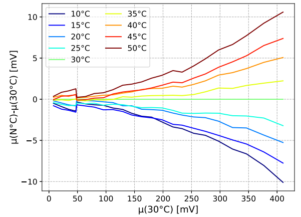
Fig. 10. Temperature dependence of the effective threshold for group 1 in SN0001. The jump at 50 mV originates from a change < 2048 to > 2048 in PMTref4.
