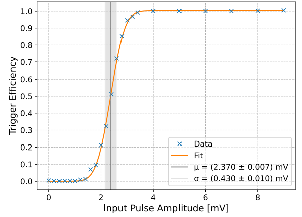
Fig. 8. Sigmoidal curve for a Thresh 2800 and PMTref4 2020 on SN0002. The input pulse amplitude is the sum of all four input channels of the trigger group.
