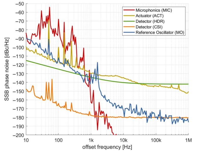
FIG. 6. Measured absolute phase noise of the relevant rf control subsystems. The measurement resolution of the CSI is 112 as within the bandwidth of [10 Hz, 1 MHz] and 64 as within the closed-loop bandwidth of 40 kHz, respectively.
