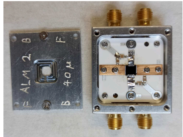
Figure 3 One of the diamond sensors mounted on a custom-designed ceramic carrier board in a metal housing.
