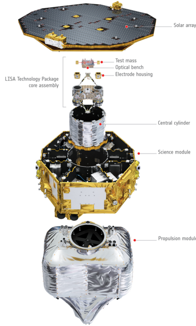
Figure 5.4: Exploded view of LPF showing the science module containing the test masses in its centre as well as the propulsion module. The technology package contains all of the experimental setup relevant to our analysis but since the entire mass of the SC goes into the calculation, we cannot completely ignore the structure or the solar panel. For simplicity, we will just perform a conservative estimate (see text). Image by ESA/ATG medialab (with permission).
