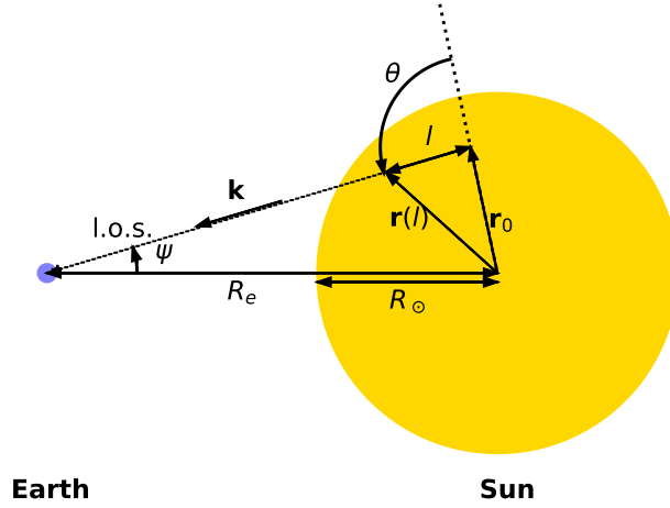
Figure 3.1: Sketch of the Sun-Earth system (adapted from Ref. [103]), where all geometric quantities necessary to calculate the solar DP flux are defined. Assuming that the Sun is to good approximation isotropic, the angular flux will only depend on the angle \psi under which the Sun is observed.
