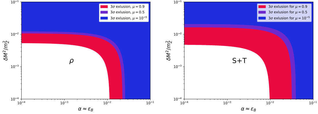
Figure 2.1: Left : 3\sigma exclusion limits of the kinetic mixing, parameterised by \alpha \approx \epsilon_B , and the mass mixing, expressed as \delta M^2/m_Z^2 , for three different DP masses parameterised by \mu = 10^{-5} (blue), 0.5 (purple), 0.9 (red). The limits are derived from the \rho parameter. Right : Analogous limits based on the S and T parameters.
