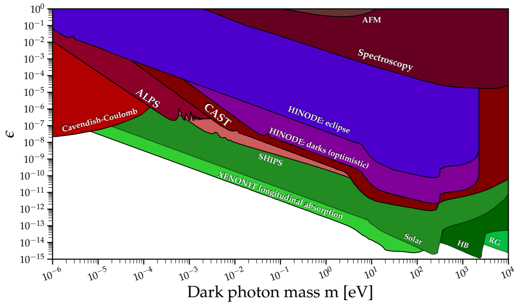
Figure 3.14: Same limits as in figure 3.9, but focusing only on the strongest and thus most optimistic limits obtained in this work, i.e. using the data-driven background subtraction, in comparison to other competing DP bounds. The plot design is taken from the outstanding repository for DP and axion-like particle (ALP) bounds by Ciaran O'Hare Ref. [162], see also Ref. [72] for a compilation of many of these limits. Generically, green contours are driven by the astrophysical production of DPs, whereas red bounds are often based on various lab-based experiments.
