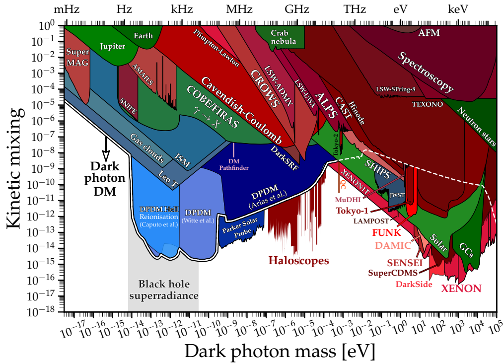
Figure 4.5: Exclusion limits of many DP(DM) searches [162]. Note that it is not immediately apparent from this plot which curves exclude the existence of DPs and which only bound the interactions of DPDM. We thus refer to our small review in this thesis, the GitHub repository itself, or Ref. [72] which covers a good explanation of many limits which however misses several recent developments.
