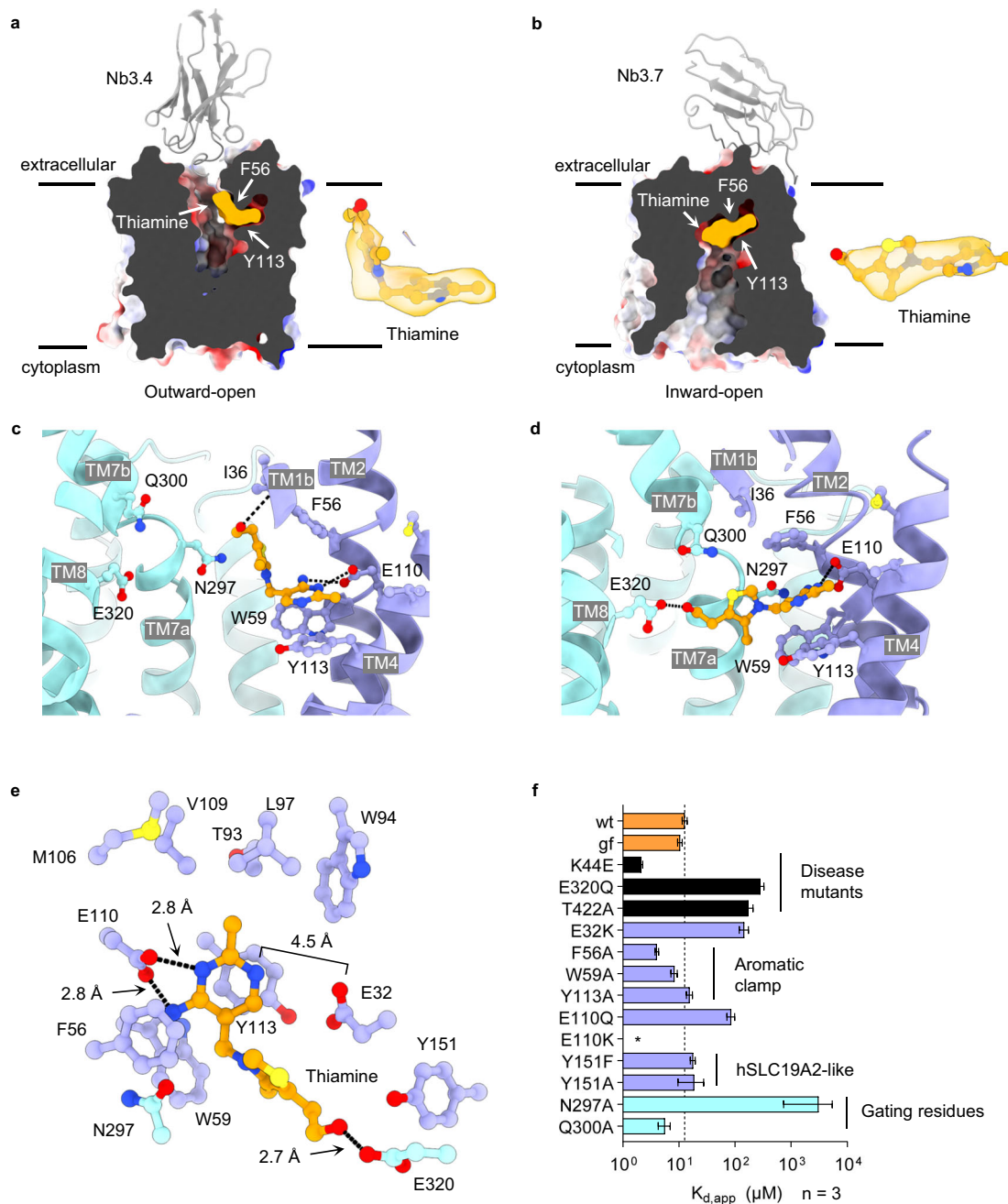
Fig. 2 | Thiamine binding site of hSLC19A3. a Localisation of the thiamine binding site of hSLC19A3 in the outward- and (b) , inward-open conformation of the transporter. The transporter is shown in electrostatic surface representation. Density for thiamine (orange) is shown separately (ChimeraX contour levels: 0.547 and 0.148, Q-scores: 0.45 and 0.57). c Residues involved in thiamine coordination in the outward- and (d) , inward-open conformation of hSLC19A3, shown in the membrane plane. e Extracellular view of hSLC19A3 highlighting the thiamine-coordinating residues in the substrate binding site of the transporter. Residues of the NTD are
