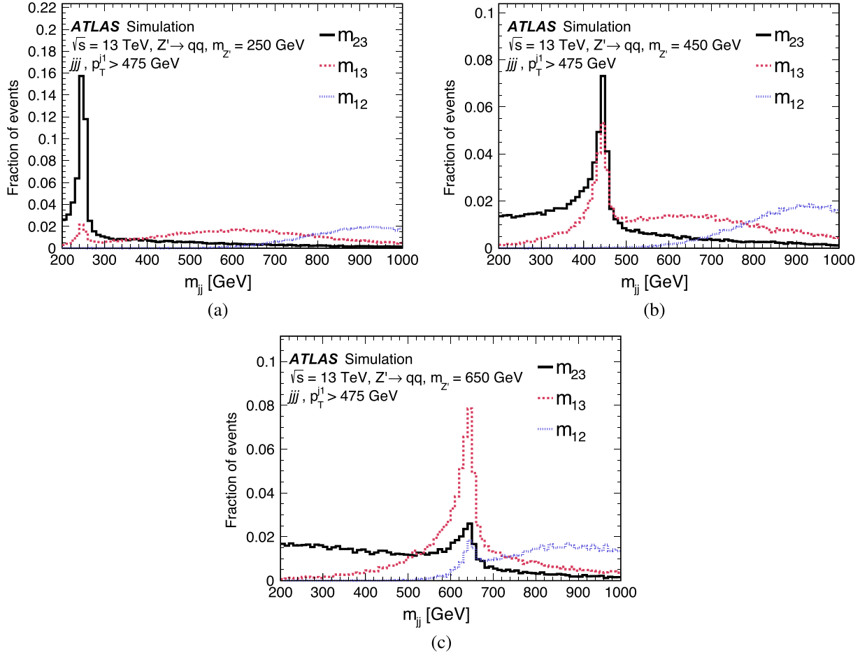
FIG. 1. Distributions of particle-level dijet mass in simulated Z' \rightarrow qq events corresponding to different combinations of two jets, where jets 1,2 and 3 correspond to the leading, subleading and third-leading jets. Signal events generated with (a) m_{Z'} = 250 GeV, (b) m_{Z'} = 450 GeV, and (c) m_{Z'} = 650 GeV are shown.
