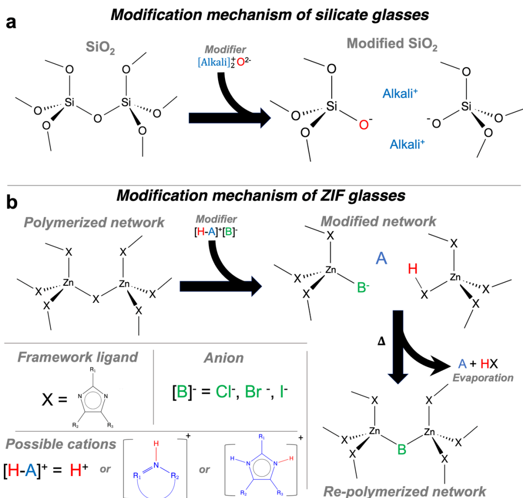
Fig. 4: Proposed mechanism of modification for ZIF glasses using halide salts. a , Well-established mechanism of modification of archetypical silicate glasses using alkali oxides. b , Proposed halide salt modification mechanism of ZIF glasses. Addition of the halide salt partially breaks up the Zn-ligand-Zn bridges to form depolymerized structures, while further heating induces the evaporation of the linker species and subsequent formation of halide-bridged Zn centers.
