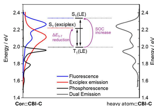
Figure 7. Schematic state diagram derived from spectroscopic data showing the different mechanisms (purple) for the increase of k_{\text{RISC}} and \Phi_{\text{TADF}} in CorCCBI-C and heavy atomCCBI-C under the approximation of identical S_0 energy levels of CBI and guestCCBI-C. Energy levels are estimated from the tangents of the emission spectra. Blue: CBI-C fluorescence at RT, red: CorCCBI-C emission at RT, black: CBI-C at 77 K with 20% ethyliodide, gray: dual emission of Pt(acac) 2 CCBI-C at RT, all in \text{CHCl}_3 under \text{N}_2 . SOC = spin–orbit coupling.
