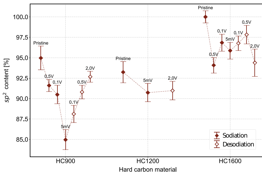
Fig. 3. sp^2 hybridized C content in pristine hard carbons carbonized at three different temperatures and in their respective ex situ negative electrodes stopped during the sodiation and desodiation of the battery. The dashed line connecting the points is shown to group the samples with the same HC material, the label denotes the voltage at which the battery was stopped, full markers represent sodiation, empty represent desodiation. The relative intensities were normalized to the intensity of the pristine HC1600 sample with the highest amount of sp^2 hybridized C.
