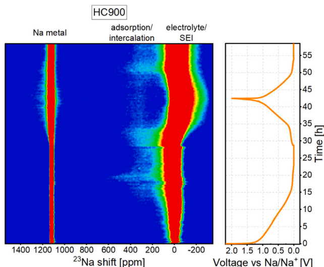
Fig. 10. Spectrum of solid-state ^{23}\text{Na} operando NMR on a Na-HC900 half-cell at 90° orientation of electrodes with respect to the external magnetic field of the spectrometer. Electrochemistry is added on the right.
