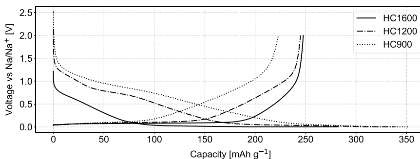
Fig. 1. The sodiation and desodiation profile of Na-ion battery with hard carbon negative electrode carbonized at 900, 1200 and 1600 °C respectively.
