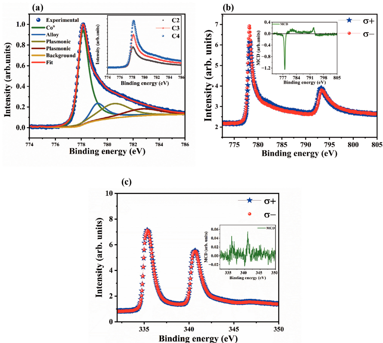
Figure 2. a) HAXPES spectra of sample C3 – Ta(4 nm)/Pd(4 nm)/Co(0.6 nm)/Pd(2 nm) for Co 2p_{3/2} ; inset shows the raw data for the samples C2, C3 and C4 b) MCD-HAXPES obtained for C6 – Ta(4 nm)/Pd(4 nm)/Co(1.5 nm)/Pd(2 nm) at the Co 2p edge; inset shows the MCD c) MCD-HAXPES obtained for C6 – Ta(4 nm)/Pd(4 nm)/Co(1.5 nm)/Pd(2 nm) at the Pd 3d edge; inset shows the MCD.
