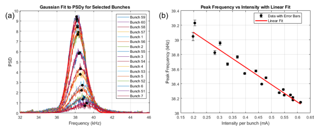
Figure 11: (a) Gaussian fit to PSDy (b) Fit to tune for selected bunches.
