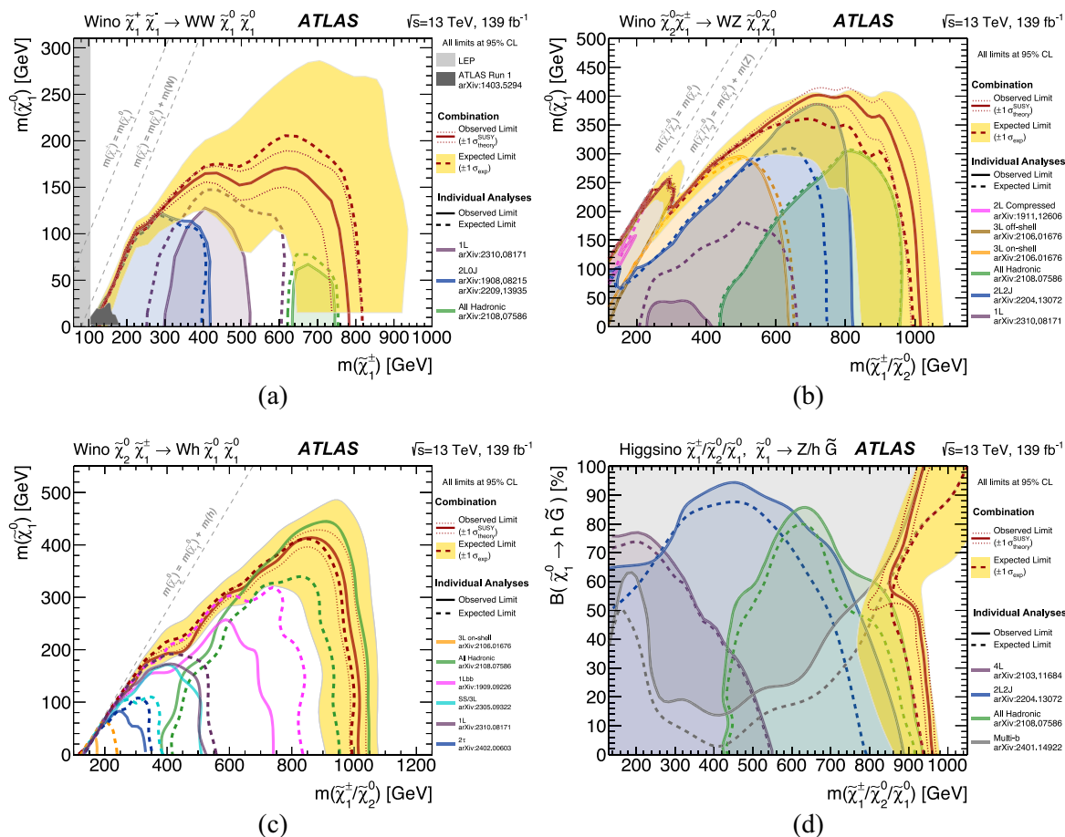
FIG. 2. The expected (dashed) and observed (solid) 95% C.L. exclusion limits on (a) chargino-pair production decaying via W bosons, (b) chargino-neutralino production decaying via W and Z bosons, (c) chargino-neutralino production decaying via W and h bosons, (d) Higgsino GGM scenarios. The limits are set using a statistical combination of searches targeting each SUSY scenario. Limits obtained by individual searches are overlaid.
