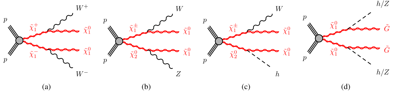
FIG. 1. Diagrams of the processes in the simplified SUSY models considered in this Letter: (a) wino chargino-pair production decaying via W bosons, (b) wino chargino-neutralino production decaying via W and Z bosons, (c) wino chargino-neutralino production decaying via W and h bosons, and (d) Higgsino GGM scenarios. In (d) the \tilde{\chi}_1^0 may be produced via \tilde{\chi}_1^+\tilde{\chi}_1^- , \tilde{\chi}_1^\pm\tilde{\chi}_{1,2}^0 , or \tilde{\chi}_1^0\tilde{\chi}_2^0 production. The gray blob represents all possible intermediate states. For these simplified models, all other SUSY particles are assumed to be heavy and decoupled.
