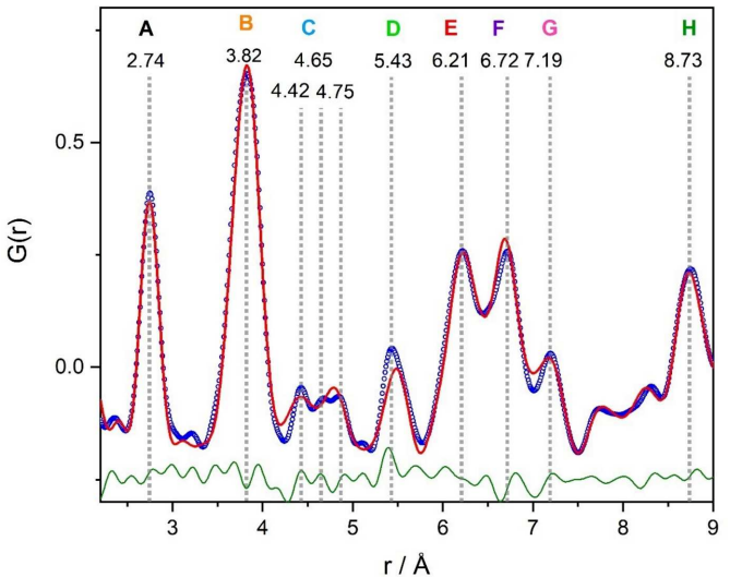
Figure 5 Real-space Rietveld refinement G(\text{calc}) of the P2_1/m structural model compared with the PDF data G(\text{obs}) . The difference function G(\text{diff}) is displayed in green.
