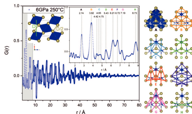
Figure 4 PDF with magnification of the local part r < 9 Å (gray area); all given distances are in Å. Corresponding distances of edge-sharing CrTe 6 octahedra are depicted on the right (view onto the b - c plane). Peak A represents Cr-Te bonds of CrTe 6 octahedra. Inset top left: schematic view onto the a - c plane. Included are Cr-Cr distances corresponding to peak D that could not be marked in the view on the right. Included in peak D are also short Te-Te distances interconnecting the chains of edge-sharing octahedra (yellow). They are short, only 2.78 Å ( r \sim D/2 ), indicating the presence of Te 2 2- polyanions (Canadell et al. , 1992).
