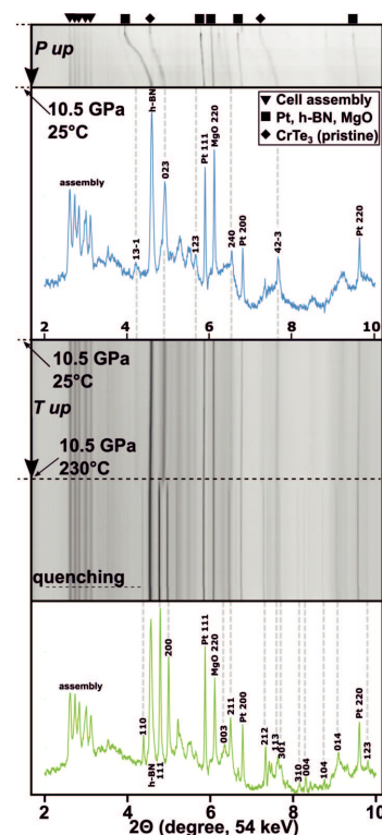
Figure 1 (a) Schematic compilation of diffractograms revealing the in situ phase transformation of the pristine CrTe 3 phase to a novel high-pressure phase at 10.5 GPa and 230°C. Note that the shift of the reflection positions from the pristine CrTe 3 and pressure markers to higher 2θ values was caused by pressures exceeding several GPa.
