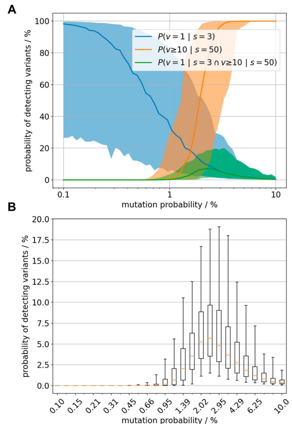
Figure 6. (A) Likelihood of observing 1 variant out of 3 sequenced samples (blue) and 10 out of 50 sequenced samples (orange) shown by the median value (bold line) and the 90% credibility interval (shaded area). The probabilities are estimated for varying rate of variants' emergence (x-axis, log scaled). The green graph represents the joint distribution i.e. the probability to observe both sample outcomes with constant variants' emergence rate. (B) Distributional details of the green graph i.e the joint probability.
