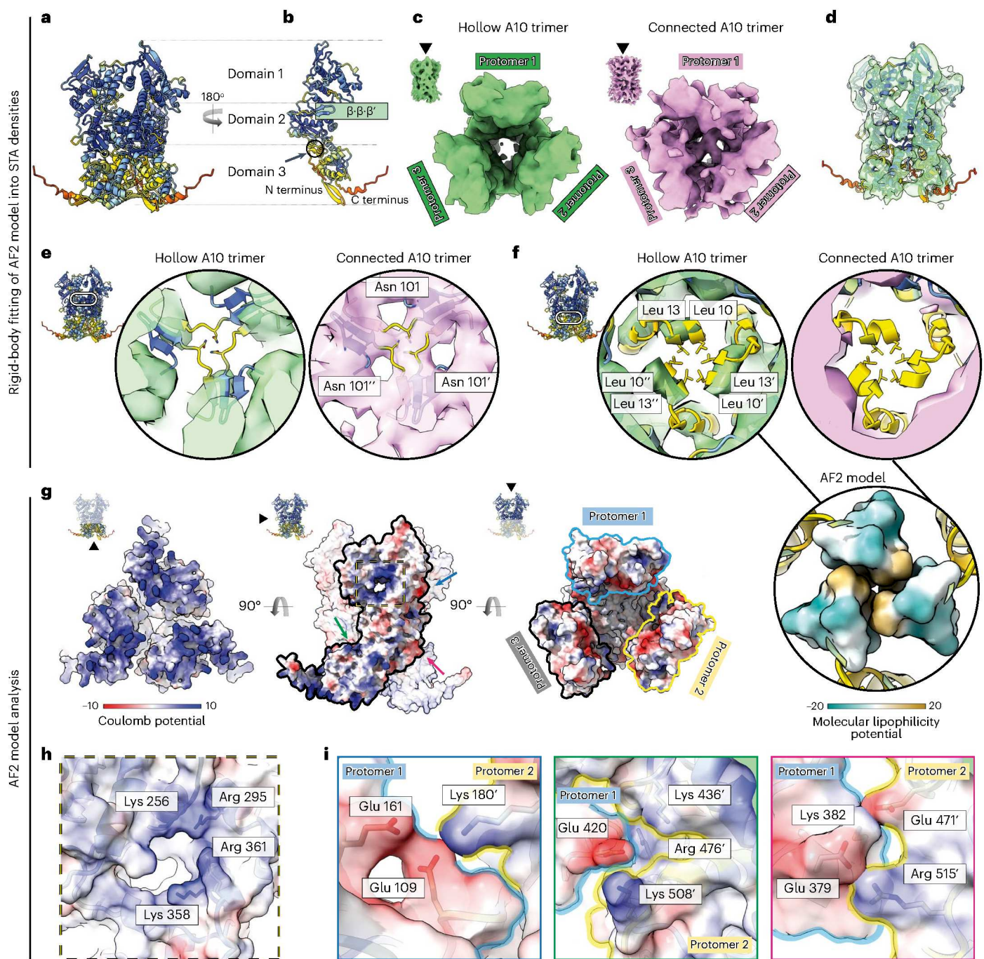
Fig. 2 | Classification and structural analysis of the A10 protein. a , AF2 prediction of the A10 trimer colored by per-residue confidence score (pLDDT) between 0 (red) and 100 (dark blue). b , Interface view of an individual protomer from the AF2-predicted A10 trimer. The \beta -strands that correspond to the linker region of a connection trimer are highlighted with the green rectangle and labeled as \beta - \beta ', referring to a putative \beta -sheet composed of two \beta -strands from one protomer and one \beta -strand from another protomer. The black arrow and the circle indicate the location of an \alpha -helix that forms putative interprotomer hydrophobic interactions at the domain 3 region. c , STA of the two distinct A10 trimer classes, hollow (green) and connected (pink). d , AF2-predicted model of A10 trimer, rigid body-fitted into the STA map of a hollow trimer. e , STA maps of the hollow (left) and connected (right) A10 trimers with the rigid body-fitted AF2-predicted model, sliced at the domain 2 region and showing the density at the region of putative \beta -sheet formation and interaction between Asn101
