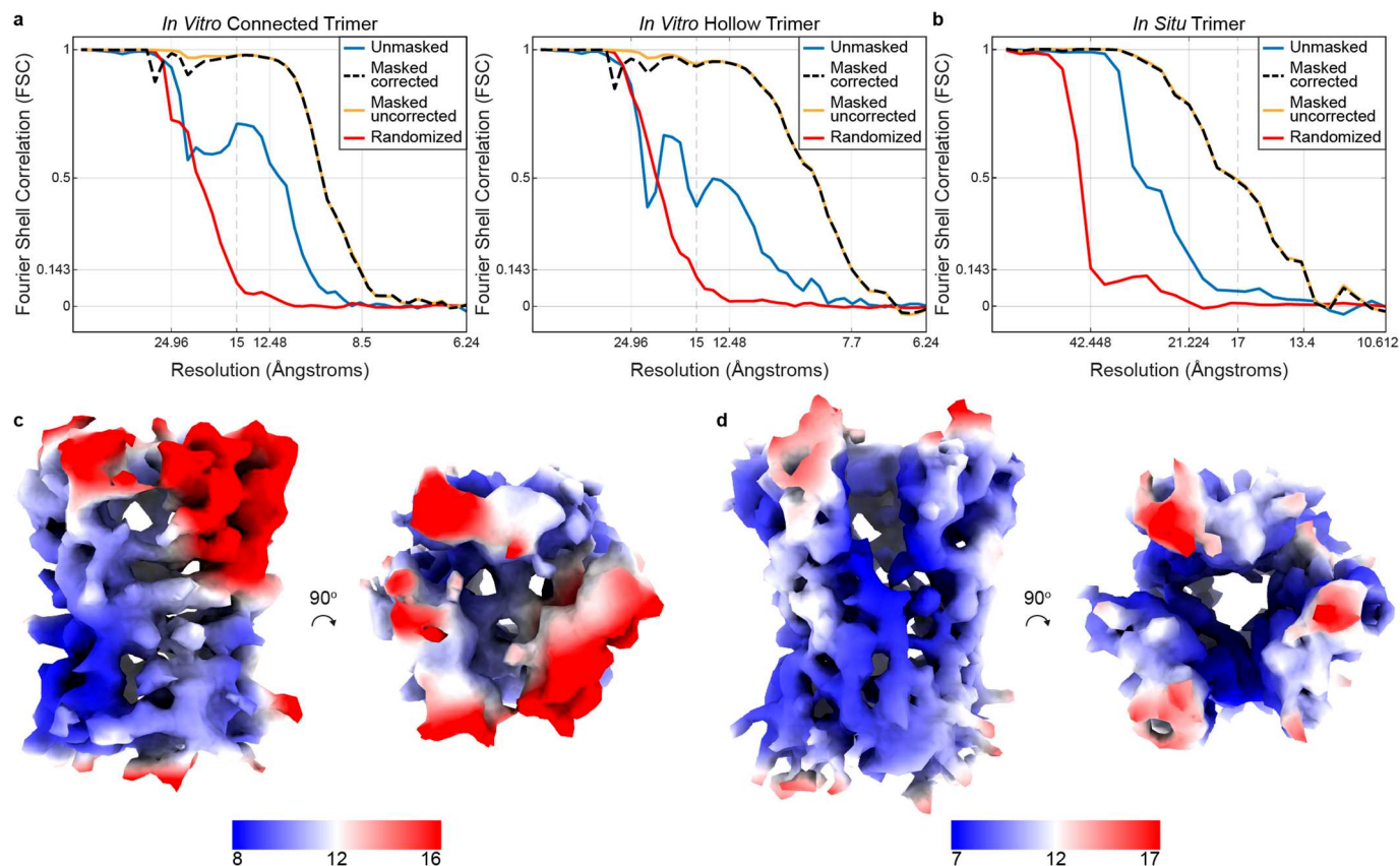
Extended Data Fig. 6 | FSC curves and local resolution maps. (a, b) Four types of FSC curves are depicted for each map. The unmasked FSC was calculated without applying a mask to the half-maps. The masked uncorrected FSC was calculated on half-maps masked with a shape mask. The randomized FSC was calculated using phase-randomization 44 . The randomized FSC was used to correct the masked uncorrected FSC which resulted in the fourth FSC curve denoted as masked corrected. The difference between the masked uncorrected and unmasked curves is caused by the dense environment of the trimers. Without the mask, the signal surrounding the average contains also signal from the neighboring trimers. Since there is no regular pattern among the neighbors, the FSC decreases at lower resolution then in the presence of the mask. The addition of the phase-randomized and mask corrected FSCs shows that the mask itself is not causing strong artifactual correlations, but instead it is focusing the
