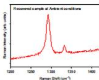
Raman spectra of diamond synthesized from hydrogenated calcite at 107 GPa
