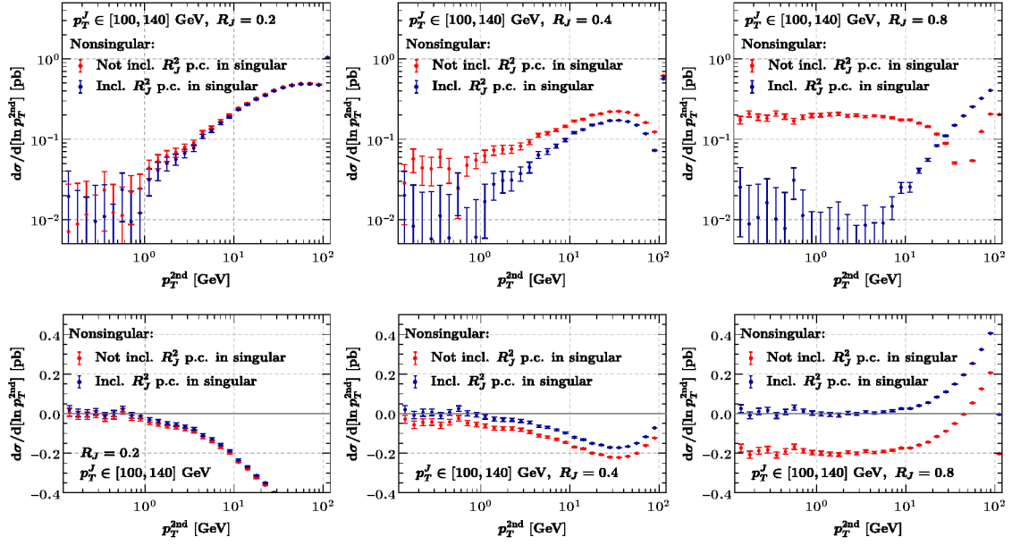
Figure 4: Nonsingular with (blue) and without (red) R_J^2 \ln p_T^{\text{cut}} power corrections for R_J = 0.2 (left), 0.4 (middle) and 0.8 (right), using log-log axes (top) and log-linear axes (bottom).
