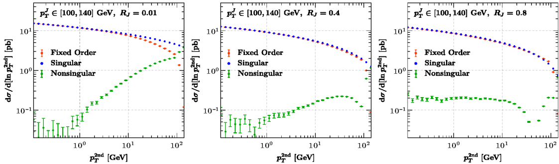
Figure 3: Full fixed order (red), singular (blue) and nonsingular (green) at NLO, differential in \ln p_T^{2\text{nd}} , for R_J = 0.01, 0.4 and 0.8 . We see that the small p_T^{2\text{nd}} behaviour of the nonsingular is linear for R_J = 0.01 and constant for large R_J , which implies the presence of R_J^2 \ln p_T^{\text{cut}} power corrections.
