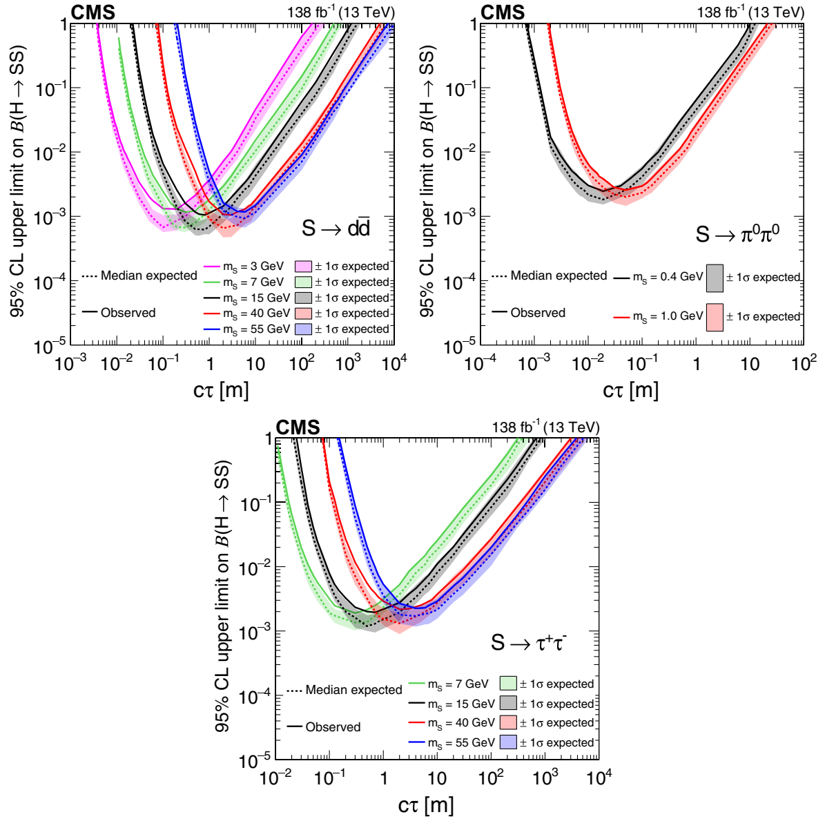
FIG. 13. The 95% CL expected (dotted curves) and observed (solid curves) upper limits on the branching fraction \mathcal{B}(H \rightarrow SS) as functions of c\tau for the S \rightarrow d\bar{d} (upper left), S \rightarrow \pi^0\pi^0 (upper right), and S \rightarrow \tau^+\tau^- (lower) decay modes. The exclusion limits are shown for different mass hypotheses.
