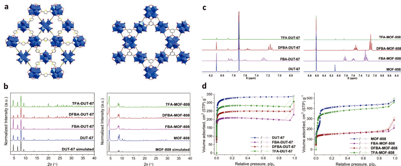
Figure 1. a) View of the main framework and pore systems in DUT-67 (left) and MOF-808 (right). Color coding: Zr polyhedral = blue, C = grey, O = red. Potentially available positions for ligand functionalization within the inorganic nodes are depicted as dark red spheres. H atoms have been omitted for clarity. b–d) PXRD data, 1 H NMR spectra, and N 2 isotherms (recorded at 77 K) of the pristine and functionalized DUT-67 and MOF-808 materials.
