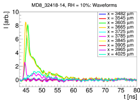
Fig. 10. Measured transient currents at different positions in the edge-region of the diode for 10% RH and V_{\text{bias}} = -900 V. The position at X = 3482 \mu\text{m} is close to the ER while the position at X = 4025 \mu\text{m} is close to the pad. The position of the GR is around X = 3700 \mu\text{m} .
