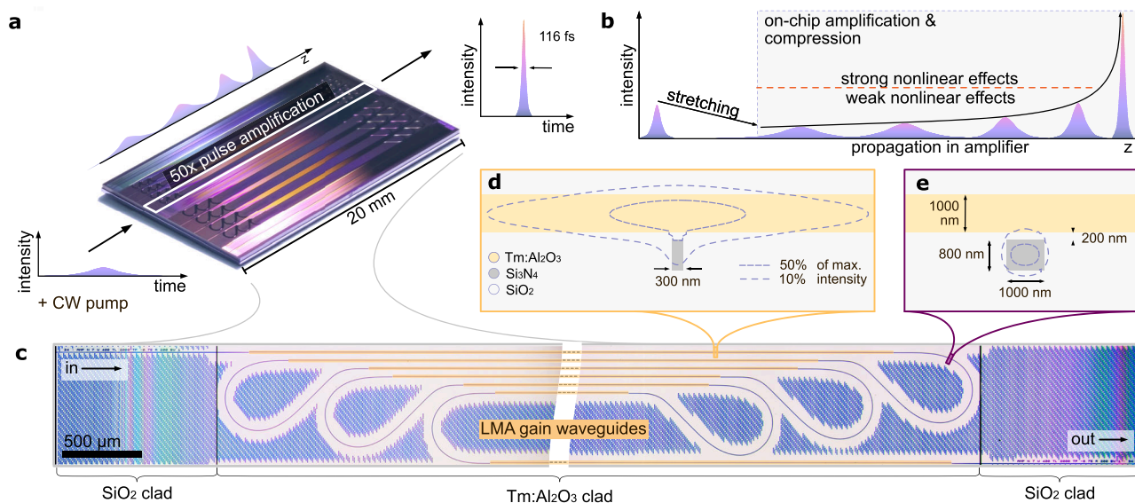
Fig. 1 | Ultrafast pulse amplification on a chip. a Photograph of the chip, hosting several amplifiers. Low-energy chirped pulses are amplified 50-fold. The output pulse is a high-peak power, nearly time-bandwidth-limited femtosecond pulse. b After temporally stretching (chirping) the input pulse, it is coupled to the amplifier chip, where it is gradually amplified and compressed, avoiding strong nonlinearities until passing the output section. c Composite photograph of an amplifier structure consisting of large mode-area (LMA) gain waveguides folded into a small 15 mm 2 -scale footprint. The waveguides are defined in a silicon nitride
