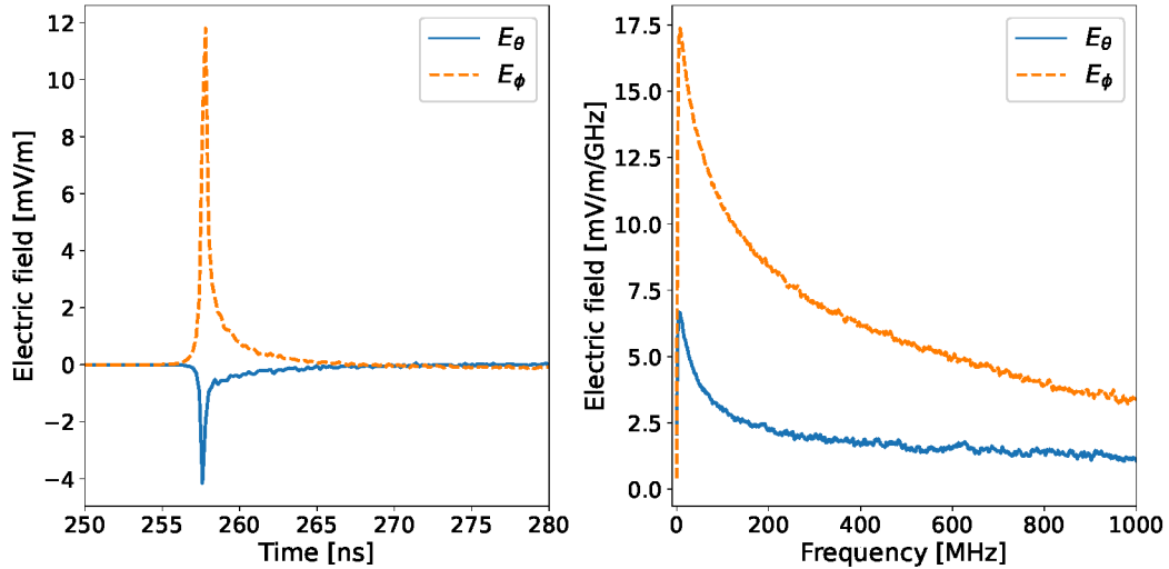
Figure 5.2: Shown are the two components E_\theta and E_\phi of the electric field generated by an air shower with energy 10^{18} eV. The left figure shows the radio pulse in the time domain. On the right the frequency spectrum is shown.
