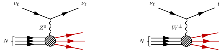
Figure 3.3: A neutrino \nu_\ell interacting with a nucleus N . Left: Neutral current (nc) interaction mediated by a Z boson, emitting a neutrino and a hadronic shower, indicated by three red lines. Right: Charged current (cc) interaction, creating a lepton \ell and a hadronic shower (indicated by three red lines).
