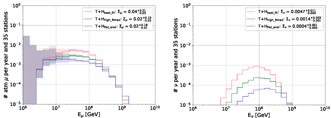
Figure 7.12: Expected event rate for muons (left) and neutrinos (right) for the same cosmic ray compositions in an RNO-G like detector with 35 station and a deep 2.5\sigma trigger. Shown are three different extra-galactic components by Heinze [229] (best fit, high maximal rigidity and flat evolution) combined with the same galactic component by Thoudam [227].
