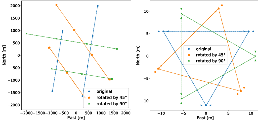
Figure 6.4: Three azimuthal rotations of the array (left) and a station (right) for 0^\circ , 45^\circ , 90^\circ . The dotted lines between the station (left) and antennas (right) are for better visibility. The three markers per antenna indicate the direction of the tines. For the simulations, only these three array geometries were used, while the antennas were randomly rotated between 0^\circ to 360^\circ to account for the different geomagnetic angles.
