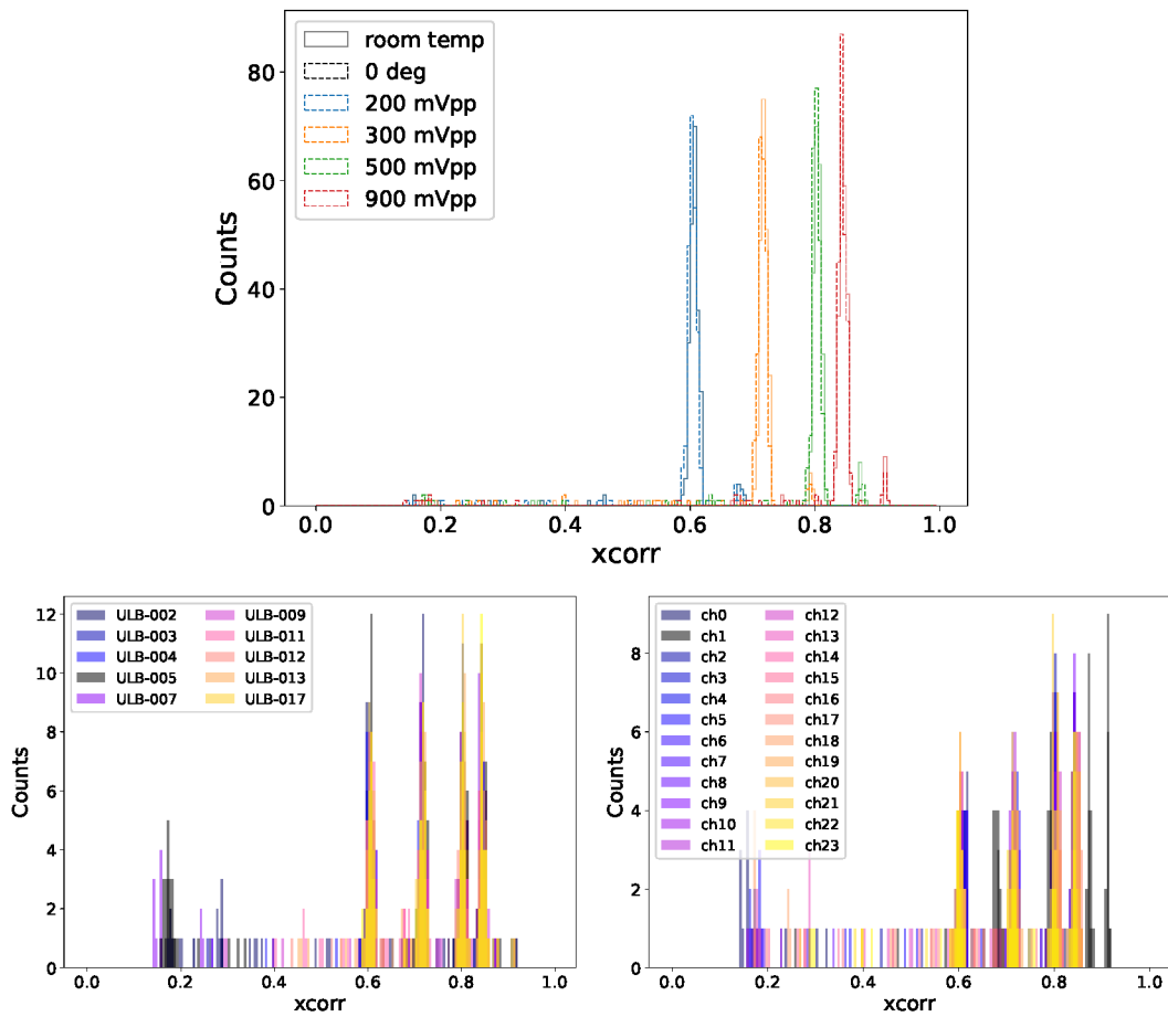
Figure 5.40: Display of the FrontEndResponse test results for all boards and channels. The cross-correlation value xcorr is calculated according to Eq. 5.13. Left: The color code differentiates the board, the data includes all temperatures and channels. Right: The color code differentiates the channels, the data includes all temperatures and boards.
