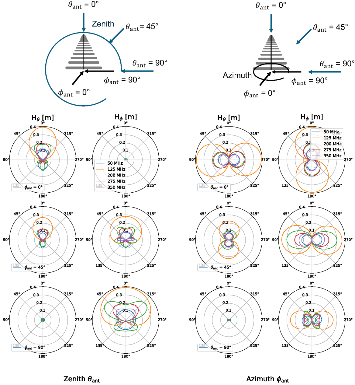
Figure 5.5: Simulated antenna response pattern of an LPDA for both polarizations in the firn. The upper left show the the zenith distribution for H_\theta (first column) and H_\phi (second column) at three different azimuth angles as stated in the legend on the left polar plot. The lower right three rows show the azimuth distribution for three different zenith angles ( 0^\circ , 45^\circ and 90^\circ ). The color code indicates the frequency (50 MHz, 125 MHz, 200 MHz, 275 MHz, 350 MHz). On the opposite side a visualization of the antenna and its directions is shown.
