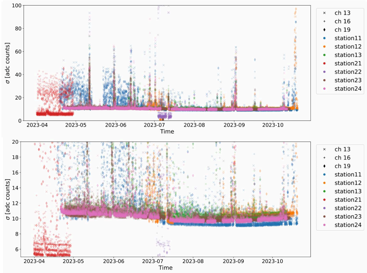
Figure 6.9: Overview of the \sigma_{\text{adc}} per run ( \sim 2 hours) in adc counts with baseline correction. About 10 000 events are shown for the 2023 season for all stations and the three upward facing LPDAs. The data is the burn sample transmitted via satellite for monitoring. All trigger types are considered. Top: \sigma in the range of 0 adc counts to 100 adc counts. Bottom: Same data but zoomed in.
