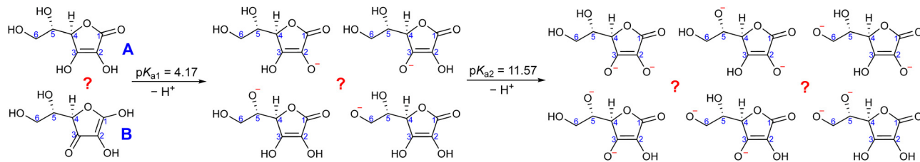
Fig. 2 Molecular structures of vitamin C in its fully protonated, singly deprotonated, and doubly deprotonated form. Two fully protonated tautomers, four hypothetical single deprotonation sites, and six hypothetical double deprotonation sites of the A tautomer are shown.
