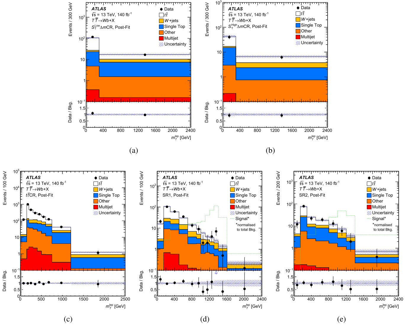
Fig. 4. Distribution for m_T^{\text{lep}} for data (dots) and predictions (histograms with various colours) in the five fit regions ((a) S_T^{\text{Low}} \Delta m\text{CR} , (b) S_T^{\text{High}} \Delta m\text{CR} , (c) t\bar{t}\text{CR} , (d) SR1, and (e) SR2, respectively) after the simultaneous fit to data under the background-only hypothesis (Post-Fit). The binning in m_T^{\text{lep}} was optimised to maximise the sensitivity to the signal in the signal regions while it is ensured that each bin of the fit regions contains a reasonable number of data events to guarantee good fit behaviour. The lower panel of each plot shows the ratio of data and predicted background yields. The arrow indicates that the ratio point is outside the ordinate range. The overflow events are included in the last bin. The error bars include the statistical uncertainty and the shaded band represents the systematic uncertainty after the likelihood fit (see text). The dashed green histograms in (d) SR1 and (e) SR2 show the shape for the signal with m_{\text{VLQ}} = 1400 GeV and \mathcal{B}(T \rightarrow Wb) = 1 scaled to the total background prediction. The expected signal event yields in each of the fit regions are displayed in Table 3.
