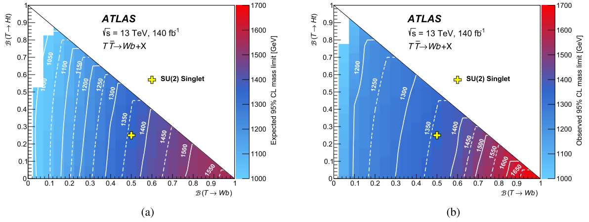
Fig. 6. (a) Expected and (b) observed 95% CL lower limits on the mass of the T -quark in the branching-ratio plane of \mathcal{B}(T \rightarrow Wb) versus \mathcal{B}(T \rightarrow Ht) . Contour lines are provided to guide the eye. The white region is due to the lower mass limit falling below 1000 GeV, the lowest signal mass considered in this search. The yellow marker indicates the branching ratio for the SU(2) singlet B scenario.
