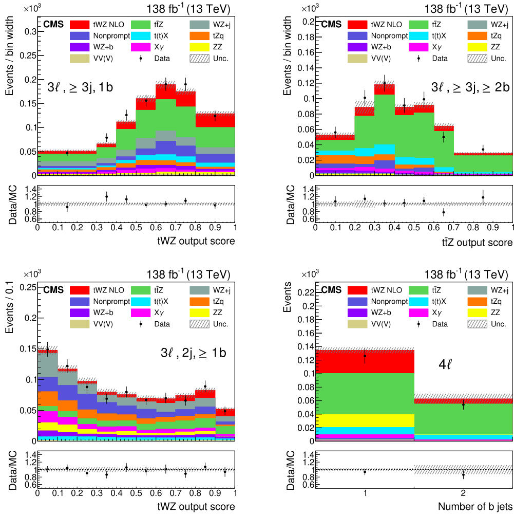
Fig. 3. Score of the t\bar{W}Z output node from the multiclass classifier in SR_{3\ell,3j} for events with exactly one b jet (upper left), and of the t\bar{t}Z output node in SR_{3\ell,3j} for events with more than one b jet (upper right); score of the t\bar{W}Z output node of the binary classifier in SR_{3\ell,2j} (lower left), and the b jet multiplicity in SR_{4\ell} (lower right). The VV(V) group in the legend denotes the VVV , WW , and W in association with jets backgrounds. The dashed band shows the total uncertainty (statistical and systematic) after the fit.
