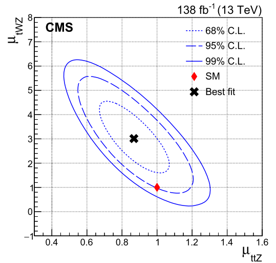
Fig. 4. Two-dimensional likelihood scan of the signal strengths of t\bar{W}Z ( \mu_{t\bar{W}Z} ) vs. t\bar{t}Z ( \mu_{t\bar{t}Z} ). The blue lines show the 68%, 95%, and 99% confidence level contours. The black cross represents the best-fit value, while the red diamond denotes the SM expectation.
