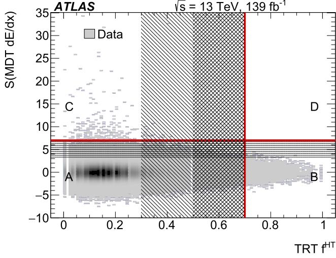
Fig. 6. ABCD plane for the z > 2 case used to assess the systematic uncertainty in the expected number of background events. Entries inside the ‘masked regions’ (here with 0.3 < f^{\text{HT}} < 0.7 , 0.5 < f^{\text{HT}} < 0.7 , and 3.0 < S(\text{MDT } dE/dx) < 7.0 , shown by the different hatch styles) do not contribute to the background estimate.
