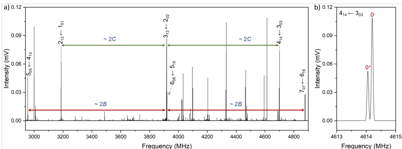
Fig. 4 a) Section of the rotational spectrum of xanthenes recorded in the 2-8 GHz frequency range, displaying the typical spectral pattern observed for b -type transitions of a near-prolate asymmetric top. Transitions have been marked using the J_{K_a,K_c} notation, where J is the quantum number representing the total angular momentum, and K_a and K_c represent the projections of the angular momentum onto the a and c axes in the limiting case of prolate and oblate symmetric tops, respectively. b) Highlight of the transition 4_{1,4} \leftarrow 3_{0,3} revealing the tunneling splitting caused by the butterfly-like motion. The two components of the tunneling splitting have been marked using the notation 0^+ and 0^- .
