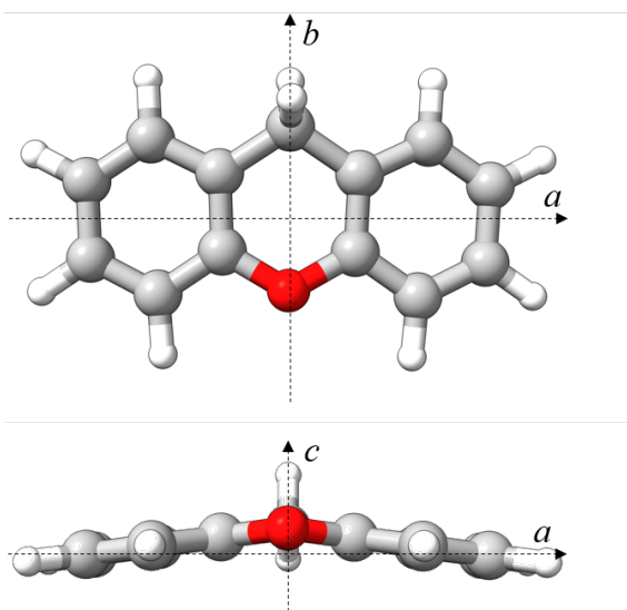
Fig. 1 Molecular structure of xanthene calculated at the B3LYP-D3BJ/def2-TZVP level of theory in a top ( ab ) and front ( ac ) view. Rendered using UCSF ChimeraX software. 35
