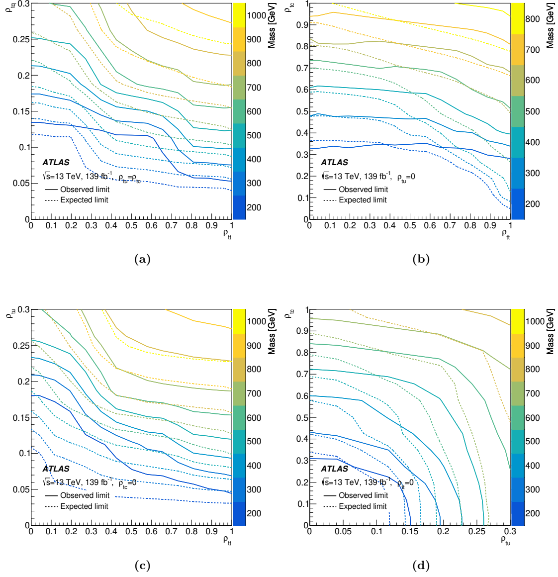
Figure 15. Observed (solid line) and expected (dashed line) exclusion limits on the scalar mass as a function of the coupling for different assumptions: (a) \rho_{tc} = \rho_{tu} , (b) \rho_{tu} = 0 , (c) \rho_{tc} = 0 , and (d) \rho_{tt} = 0 .
