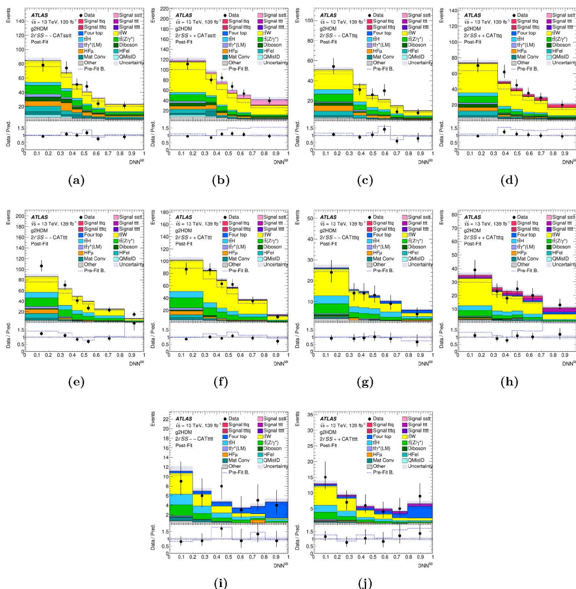
Figure 12. Comparison between data and prediction for the \text{DNN}^{\text{SB}} distribution used in different signal region categories of the 2\ell\text{SS} channel: (a) 2\ell\text{SS} \text{ --- CAT sstt} , (b) 2\ell\text{SS} \text{ ++ CAT sstt} , (c) 2\ell\text{SS} \text{ --- CAT ttq} , (d) 2\ell\text{SS} \text{ ++ CAT ttq} , (e) 2\ell\text{SS} \text{ --- CAT ttt} , (f) 2\ell\text{SS} \text{ ++ CAT ttt} , (g) 2\ell\text{SS} \text{ --- CAT tttq} , (h) 2\ell\text{SS} \text{ ++ CAT tttq} , (i) 2\ell\text{SS} \text{ --- CAT tttt} , and (j) 2\ell\text{SS} \text{ ++ CAT tttt} . The expected signal for m_H = 900 GeV and couplings \rho_{tt}=0.6 , \rho_{tc}=0.0 , and \rho_{tu}=1.1 , along with the background contributions, is shown after the likelihood fit to data (“Post-Fit”) for the signal-plus-background hypothesis. The ratio of the data to the prediction (“Pred.”) is shown in the lower panel, separately for post-fit signal-plus-background (black points) and pre-fit background (dashed blue line). The size of the combined statistical and systematic uncertainty in the signal-plus-background prediction is indicated by the blue hatched band.
