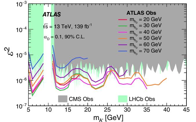
FIG. 5. Observed 90% C.L. upper limits on \epsilon^2 , assuming of \alpha_D = 0.1 , as a function of m_{A'} with different dark Higgs boson masses ranging from 20 to 70 GeV. The parameter space excluded by LHCb [12] (CMS [78]) is covered by the green (gray) shaded regions.
