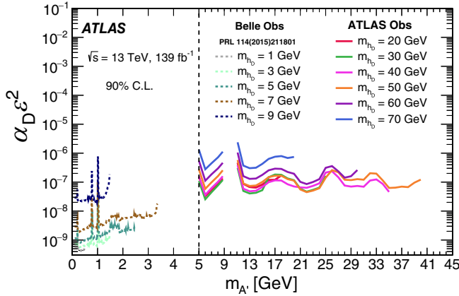
FIG. 4. Observed 90% C.L. upper limits on \alpha_D \epsilon^2 , as a function of m_{A'} with different dark Higgs boson masses, from this search (solid curves) compared with the results from Belle [15] (dashed curves).
