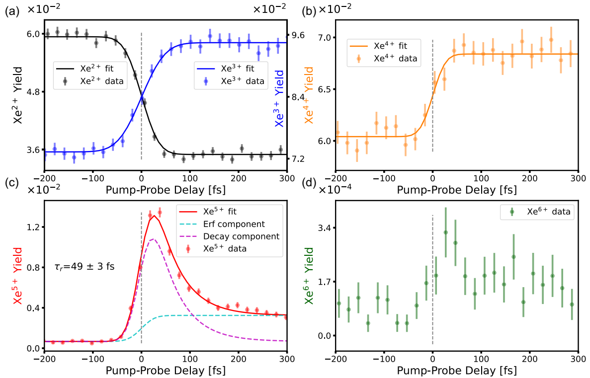
FIG. 4. (a)–(d) The ion yields of \text{Xe}^{q+} ( q = 2 – 6 ) versus delay between the 160-eV XUV pump and NIR probe. In (a) left y axis is for the yield of \text{Xe}^{2+} , and the right axis is for the yield of \text{Xe}^{3+} . The ion yields of \text{Xe}^{q+} ( q = 2 – 4 ) are fitted with a step function given in Eq. (1), yielding the cross-correlation time of (37 \pm 3) fs for \text{Xe}^{2+} , (44 \pm 5) fs for \text{Xe}^{3+} , and (31 \pm 7) fs for \text{Xe}^{4+} . The yield of \text{Xe}^{5+} in (c) is fitted with the function given in Eq. (2) with a cross-correlation time of (30 \pm 1) fs and an average lifetime of (49 \pm 3) fs. The results of the fitting procedure are described in the text, and more details are given in the Appendix. The purple and cyan fits in (c) represent the exponential and step-function components of the fit, whereas the red solid line shows the combined effect of the function.
