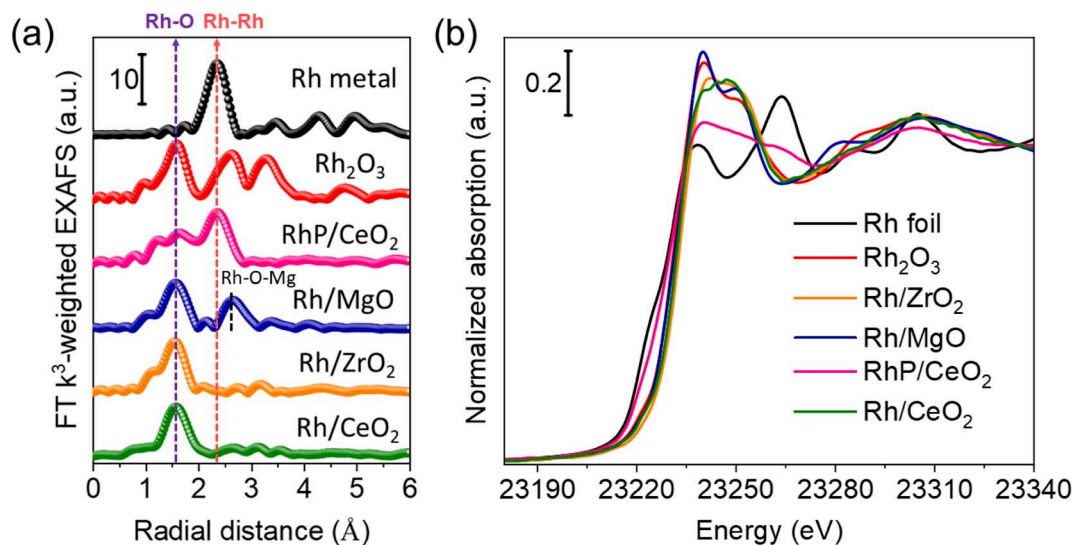
Fig. 2 (a) Fourier transform of the k^3 -weighted EXAFS spectra and (b) XANES spectra at the Rh K-edge of the Rh catalysts supported over CeO 2 , ZrO 2 , and MgO. Rh 2 O 3 and Rh foil are shown as references for comparison.
