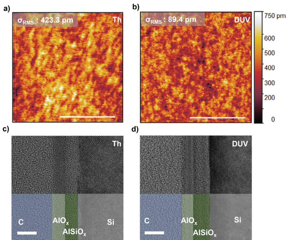
Figure 3. AFM and TEM images showing the surface morphology and thickness of as fabricated \text{AlO}_x films via a), c) thermal annealing and b), d) DUV exposure respectively. The scale bar in the AFM and TEM images correspond to 500 and 5 nm respectively. The EDS mapping for the TEM samples is included in Figure S6 (Supporting Information).
