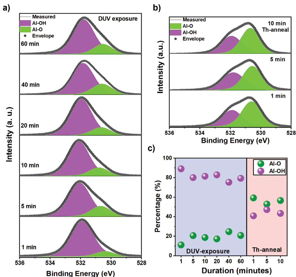
Figure 2. XPS spectra of O1s peaks for \text{AlO}_x thin films at different a) DUV-exposure and b) thermal-anneal duration. c) The calculated Al–O and Al–OH peak percentages from the peak fit analysis. The Al–O and Al–OH peaks were at 530.5 \pm 0.3 and 532.2 \pm 0.3 eV respectively.
