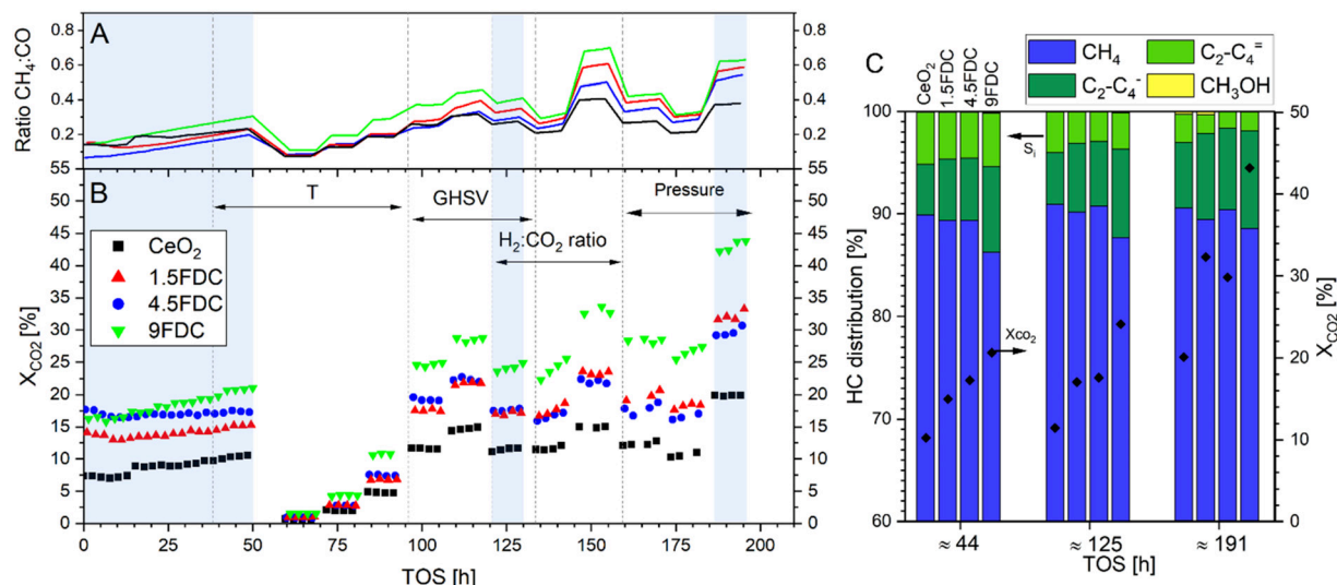
Fig. 1 Full experiment displaying the X_{\text{CO}_2} (bottom-panel B) and \text{CH}_4:\text{CO} ratio (top panel-A) with TOS for all the samples. Arrows within the bottom panel display the variation periods for specific parameters, while the regions with blue backgrounds are obtained at the same operating conditions ( 500^\circ\text{C} , \text{H}_2:\text{CO}_2:\text{Ar} = 3:1:1 , 20 bar and 50\,000\text{ mL h}^{-1}\text{ g}_{\text{cat}}^{-1} ). The detailed experimental conditions of each data point can be found in the ESI.† Panel C displays the selectivity toward HCs for all the samples in the blue regions in panel B (same operating conditions as panel B).
