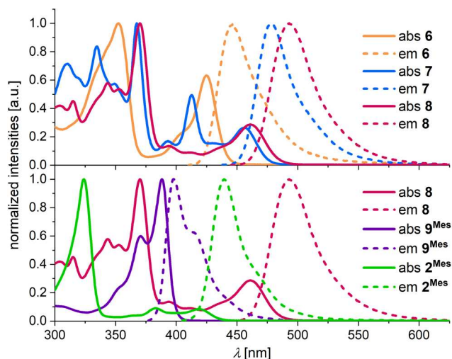
Fig. 2 Normalized UV/vis absorption and emission spectra of 6 (orange), 7 (blue), 8 (red), 9 Mes (purple), and 2 Mes (green), measured in THF.
