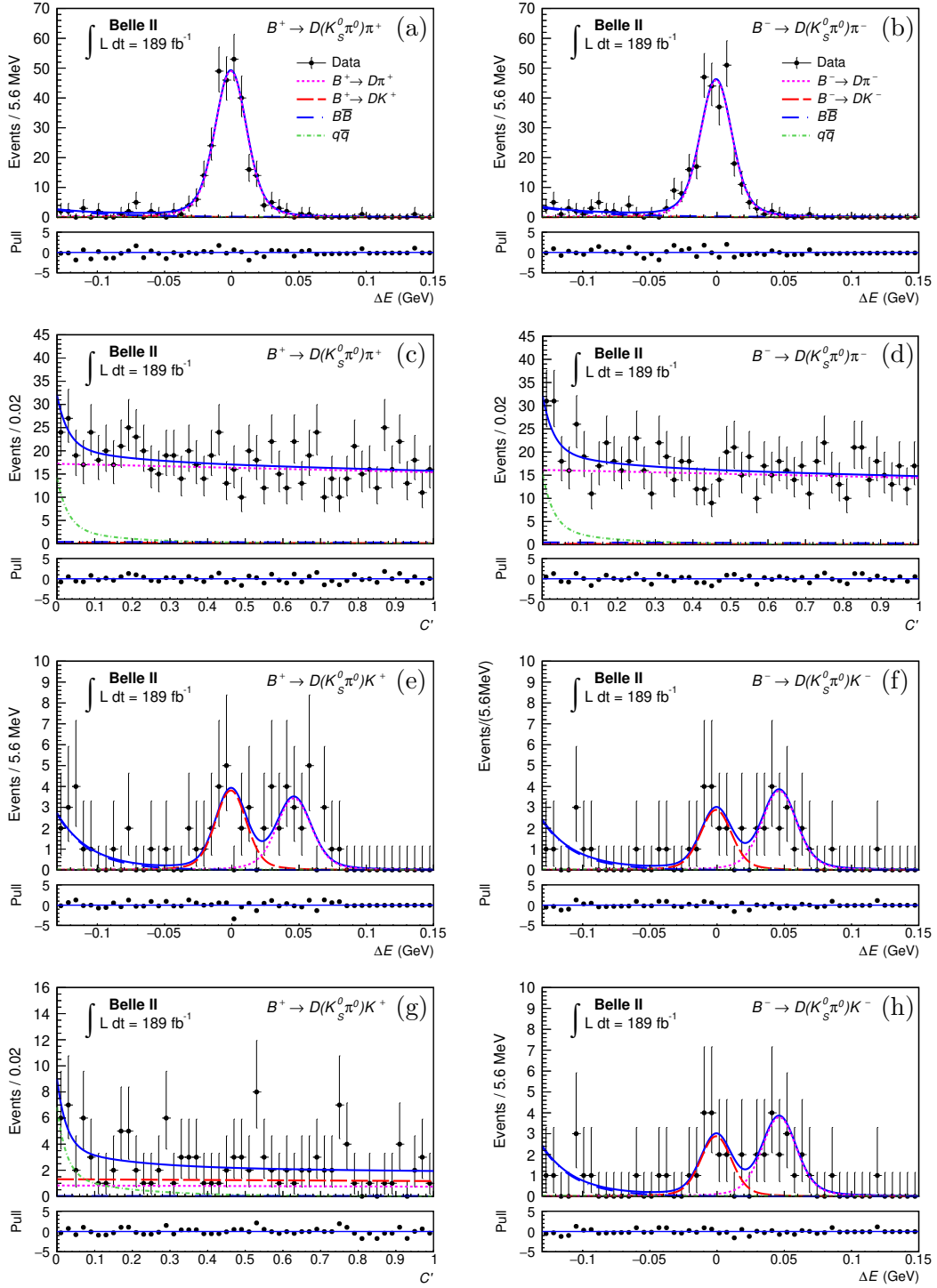
Figure 6. Distributions of \Delta E and C' for B^\pm \rightarrow D(\rightarrow K_s^0 \pi^0) h^\pm candidates in the Belle II data with fit projections overlaid. Differences between data and fit results normalized by the uncertainty in data are shown in the bottom panels.
