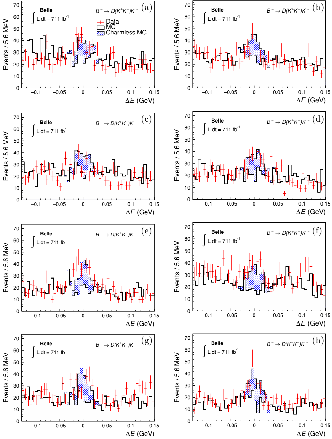
Figure 8. \Delta E distributions of B^\pm \rightarrow D(\rightarrow K^- K^+) K^\pm in Belle data and Belle simulated samples for the lower sidebands [1.67, 1.71] \text{ GeV}/c^2 (a), [1.71, 1.75] \text{ GeV}/c^2 (b), [1.75, 1.79] \text{ GeV}/c^2 (c), and [1.79, 1.83] \text{ GeV}/c^2 (d), and the upper sidebands [1.90, 1.94] \text{ GeV}/c^2 (e), [1.94, 1.98] \text{ GeV}/c^2 (f), [1.98, 2.02] \text{ GeV}/c^2 (g), and [2.02, 2.06] \text{ GeV}/c^2 (h). The red error bar is Belle data, empty histogram stands for Belle simulated sample (without charmless decays of B mesons), the filled blue histogram stands for charmless-only decays of B in Belle simulated sample.
