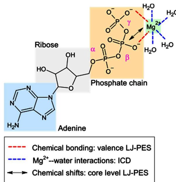
Figure 2. (a) Molecular structure of ATP (aq) in the deprotonated form (ATP 4− (aq) ), as predominantly found at physiological pH. Adenine, ribose, and \alpha -, \beta -, and \gamma -phosphate units are labeled; one of many motifs for Mg^{2+} binding is shown (see text). Molecular interactions probed using valence and core-level LJ-PES, as well as ICD spectroscopy, are highlighted using red and blue dashed lines, respectively.
