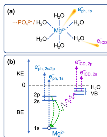
Figure 7. (a) Ejection of the initial 1s photoelectron, 1s\ e^-_{\text{ph}} , from \text{Mg}^{2+}_{(\text{aq})} and an ICD electron, e^-_{\text{ICD}} , associated with the subsequent valence ionization of a hydration-shell water molecule. The sketch also illustrates the direct interaction of \text{Mg}^{2+}_{(\text{aq})} with a phosphate unit of \text{ATP}_{(\text{aq})} which reduces the number of water molecules in the first solvation shell. (b) Energy-level diagram depicting the ICD process studied here. The open circle denotes the 1s core hole upon ionization of \text{Mg}^{2+} ; e^-_{\text{ph}} are the ejected 1s, 2s, and 2p photoelectrons. BE and KE denote electron binding and electron kinetic energies of the measured electrons, respectively. The nonlocal ICD processes, where the relaxation of the metal core hole involves the first solvation shell, lead to the ionization of all water valence (VB) orbitals (and potentially also of phosphate). This produces the ICD electrons e^-_{\text{ICD}, 2s} and e^-_{\text{ICD}, 2p} .
