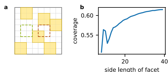
Figure 8. Fractional coverage of nonoverlapping PDPA molecules on a crystal facet depends on the facet's area. (a) The gray lattice represents a crystal facet covered by PDPA molecules (yellow squares). The PDPA molecules are not allowed to overlap (i.e., a next PDPA can occupy the green dashed square but not the red one). (b) The PDPA coverage vs the side length of a facet.
