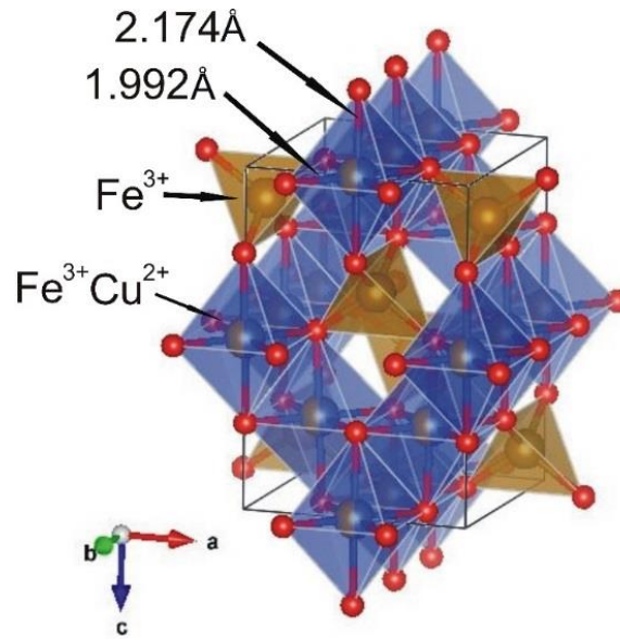
Figure 2. Crystal structure of the tetragonally distorted \text{CuFe}_2\text{O}_4 at ambient conditions.
