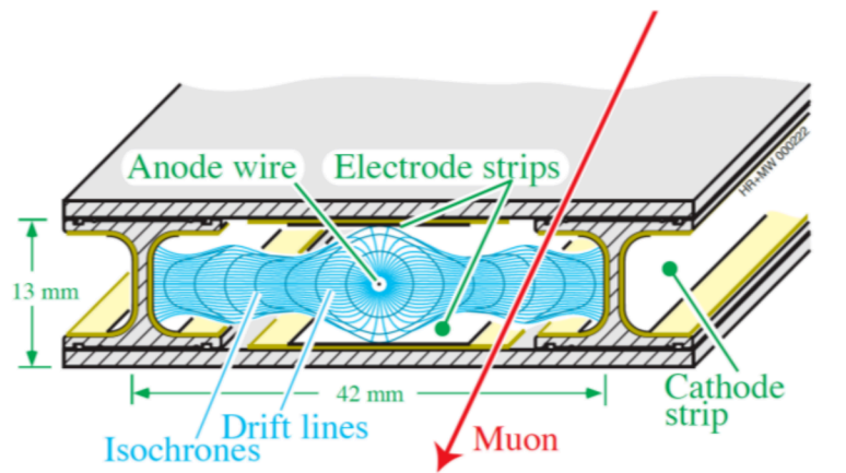
Figure 2.7: Layout of a drift tube cell. The blue lines represent the electric field in the gas volume. Taken from Ref. [54]
