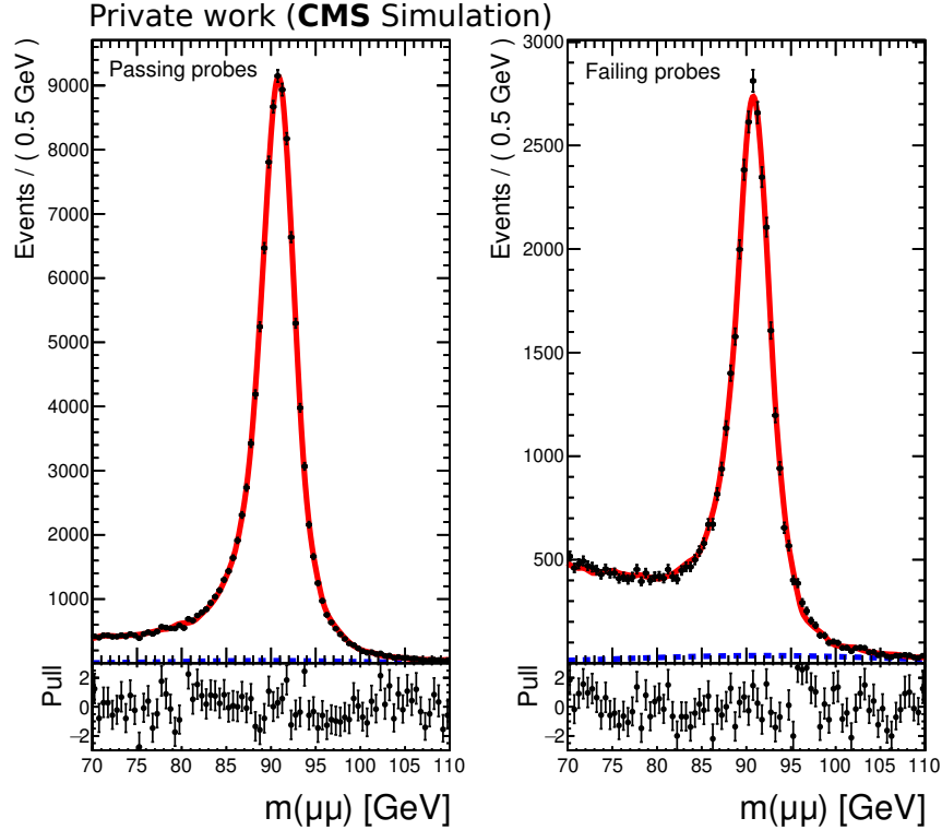
Figure 2.13: Example of tag-and-probe fit perform on the muon invariant mass in Z \rightarrow \mu^+ \mu^- events for the passing (left) and failing (right) probes. The red line indicates the signal+background model, while the blue dotted line is the background component.
